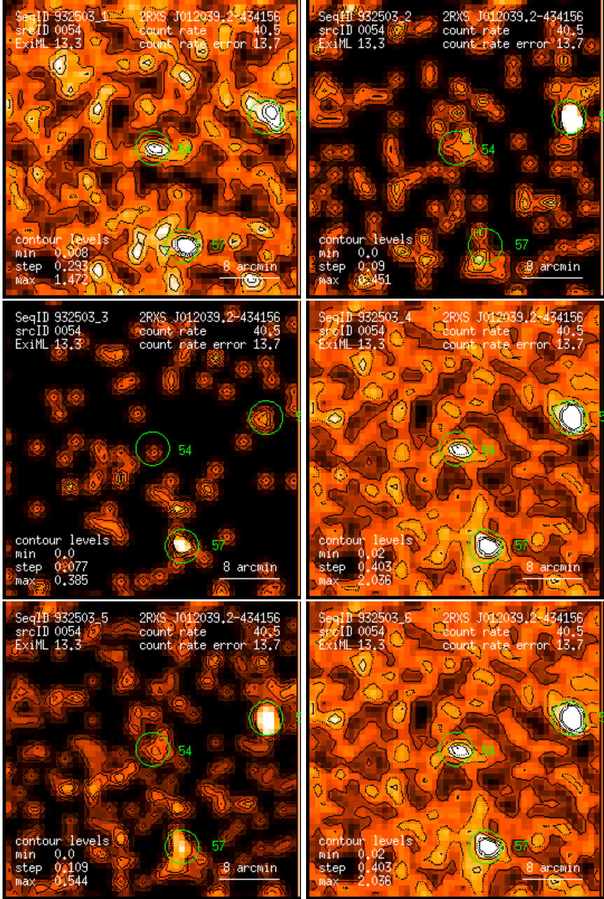
Figure 54: RASS 932503: detection 0054: band rate images, Gaussian filter: (1) PSPC channels 11 – 41, (2) 52 – 90, (3) 91 – 201, (4) 11 – 235, (5) 52 – 201, (6) 11 – 201. Broad band rates in counts/ks. Band rate contour levels in counts/ks/arcmin 2 .
