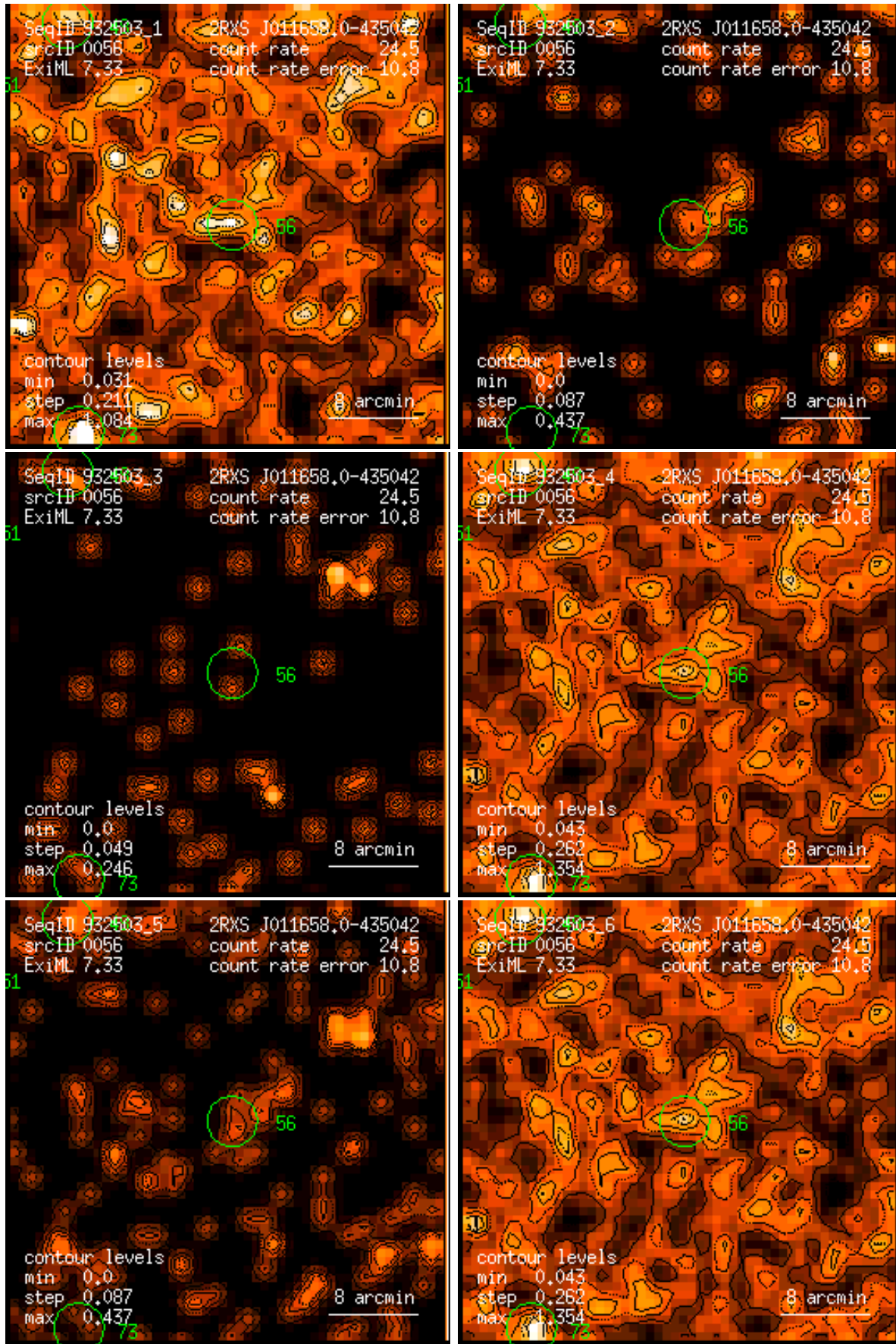
Figure 56: RASS 932503: detection 0056: band rate images, Gaussian filter: (1) PSPC channels 11 – 41, (2) 52 – 90, (3) 91 – 201, (4) 11 – 235, (5) 52 – 201, (6) 11 – 201. Broad band rates in counts/ks. Band rate contour levels in counts/ks/arcmin 2 .
