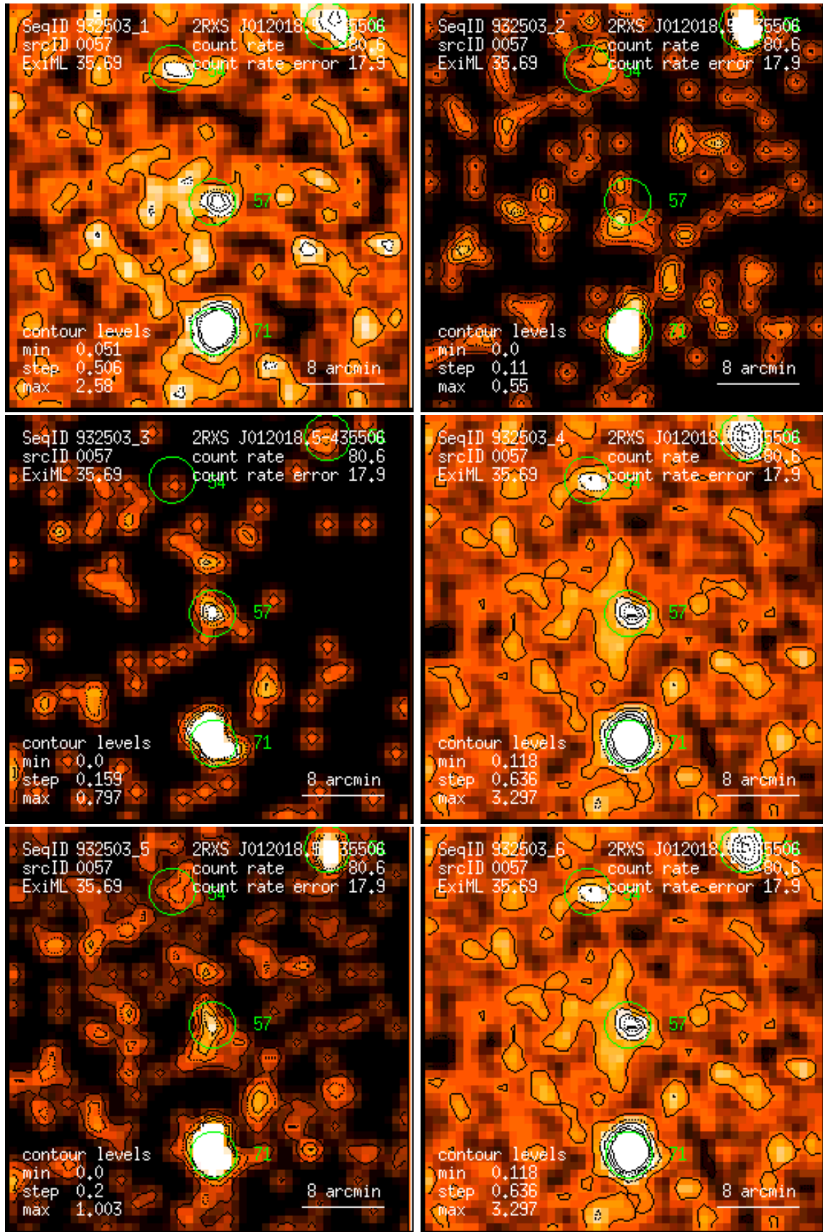
Figure 57: RASS 932503: detection 0057: band rate images, Gaussian filter: (1) PSPC channels 11 – 41, (2) 52 – 90, (3) 91 – 201, (4) 11 – 235, (5) 52 – 201, (6) 11 – 201. Broad band rates in counts/ks. Band rate contour levels in counts/ks/arcmin 2 .
