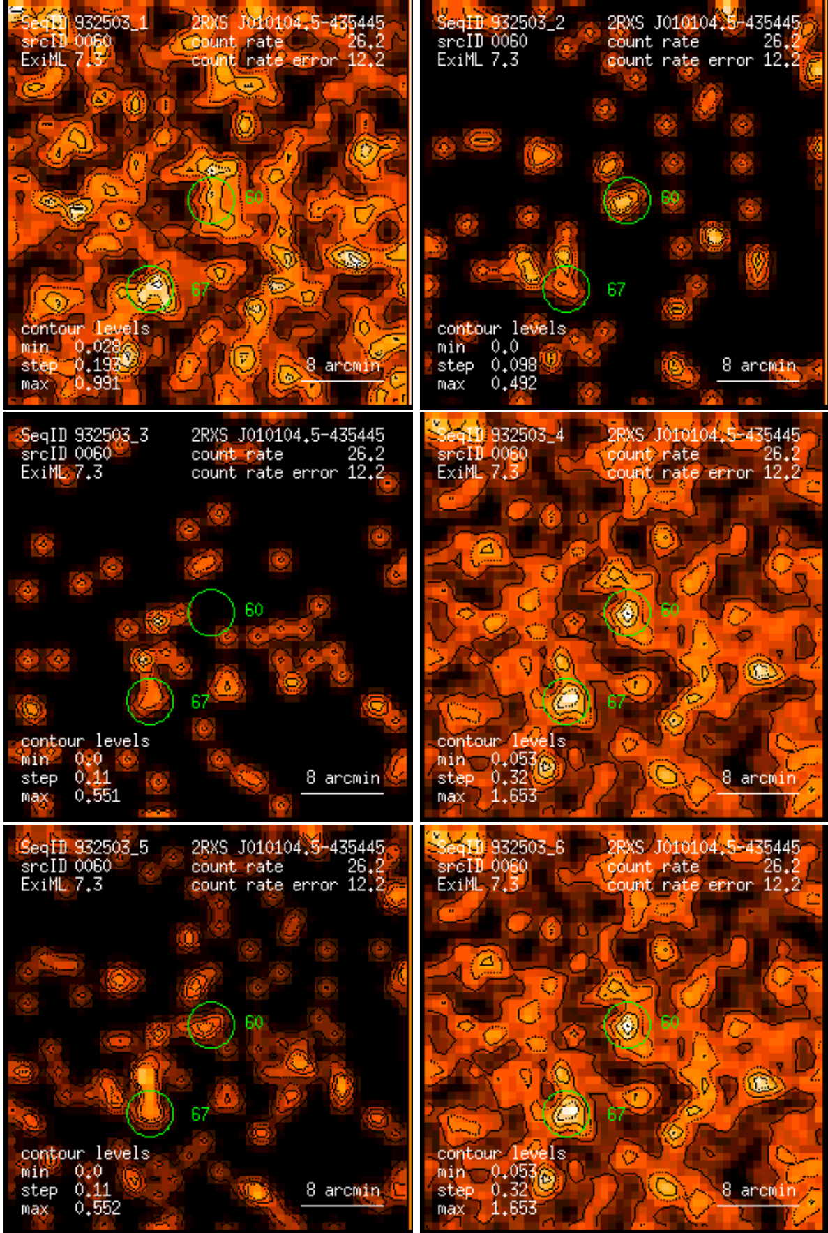
Figure 60: RASS 932503: detection 0060: band rate images, Gaussian filter: (1) PSPC channels 11 – 41, (2) 52 – 90, (3) 91 – 201, (4) 11 – 235, (5) 52 – 201, (6) 11 – 201. Broad band rates in counts/ks. Band rate contour levels in counts/ks/arcmin 2 .
