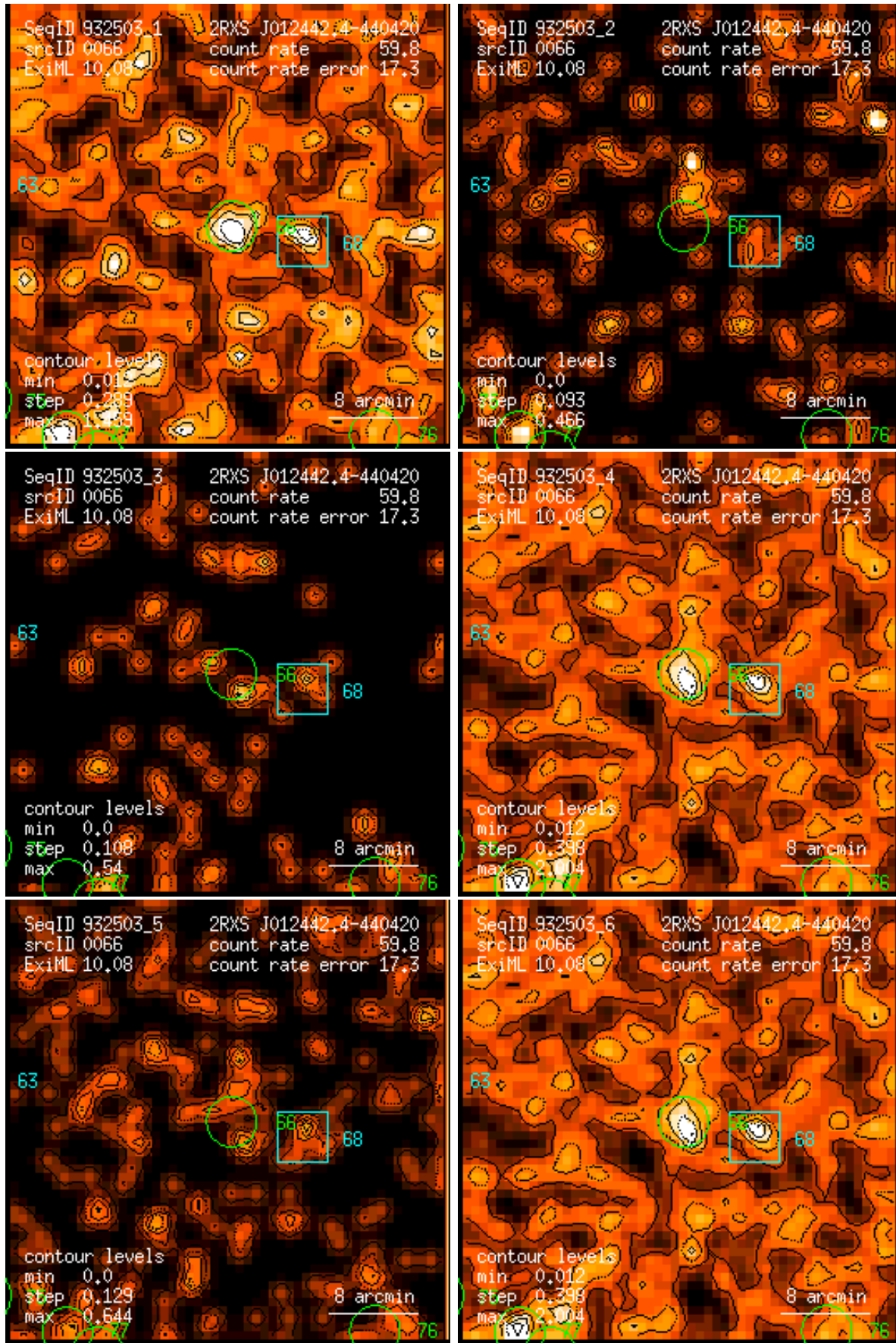
Figure 66: RASS 932503: detection 0066: band rate images, Gaussian filter: (1) PSPC channels 11 – 41, (2) 52 – 90, (3) 91 – 201, (4) 11 – 235, (5) 52 – 201, (6) 11 – 201. Broad band rates in counts/ks. Band rate contour levels in counts/ks/arcmin 2 .
