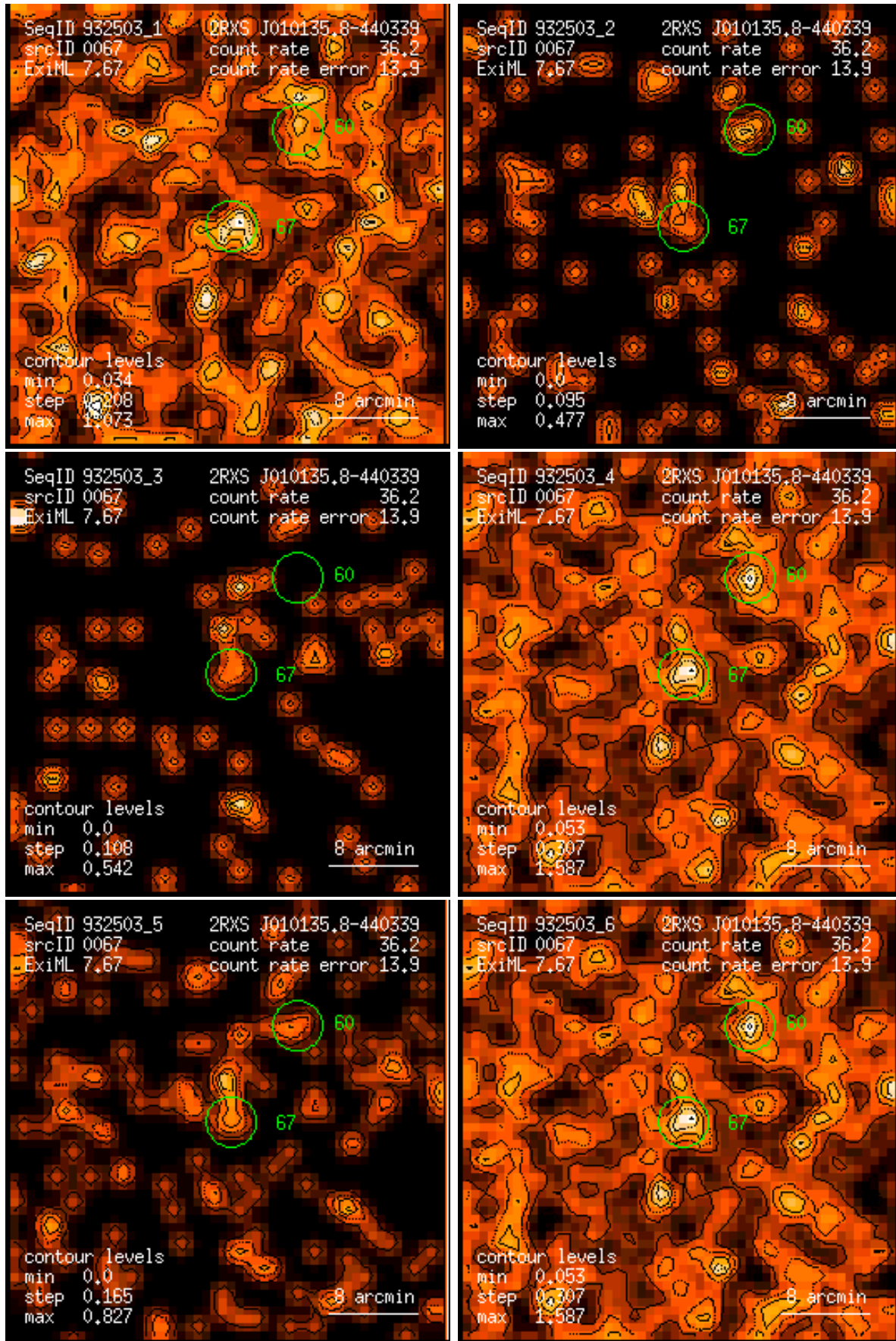
Figure 67: RASS 932503: detection 0067: band rate images, Gaussian filter: (1) PSPC channels 11 – 41, (2) 52 – 90, (3) 91 – 201, (4) 11 – 235, (5) 52 – 201, (6) 11 – 201. Broad band rates in counts/ks. Band rate contour levels in counts/ks/arcmin 2 .
