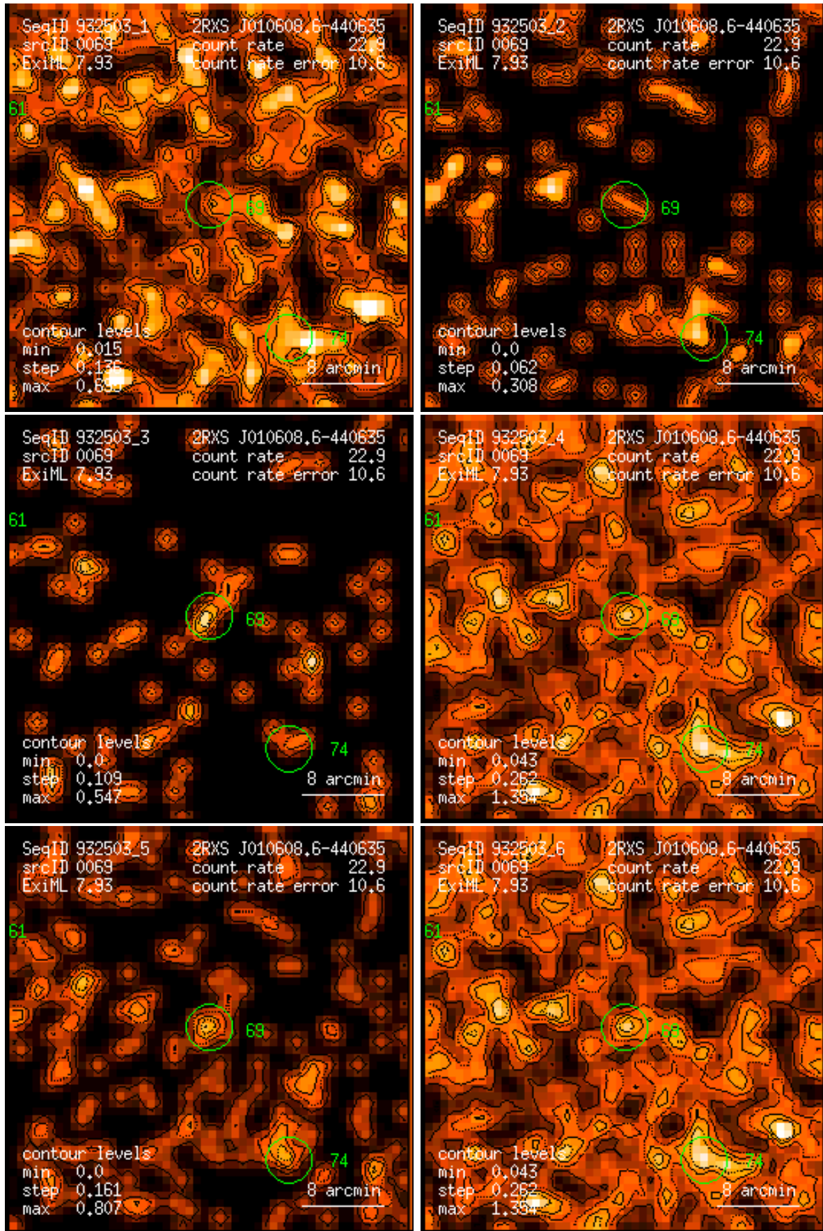
Figure 69: RASS 932503: detection 0069: band rate images, Gaussian filter: (1) PSPC channels 11 – 41, (2) 52 – 90, (3) 91 – 201, (4) 11 – 235, (5) 52 – 201, (6) 11 – 201. Broad band rates in counts/ks. Band rate contour levels in counts/ks/arcmin 2 .
