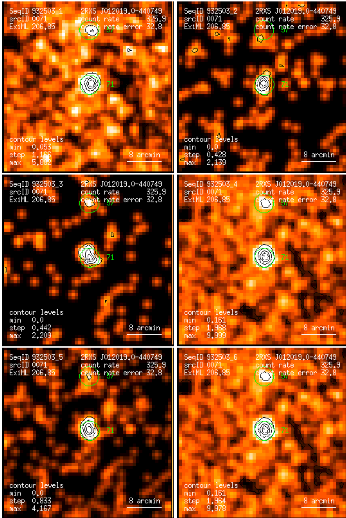
Figure 71: RASS 932503: detection 0071: band rate images, Gaussian filter: (1) PSPC channels 11 – 41, (2) 52 – 90, (3) 91 – 201, (4) 11 – 235, (5) 52 – 201, (6) 11 – 201. Broad band rates in counts/ks. Band rate contour levels in counts/ks/arcmin 2 .
