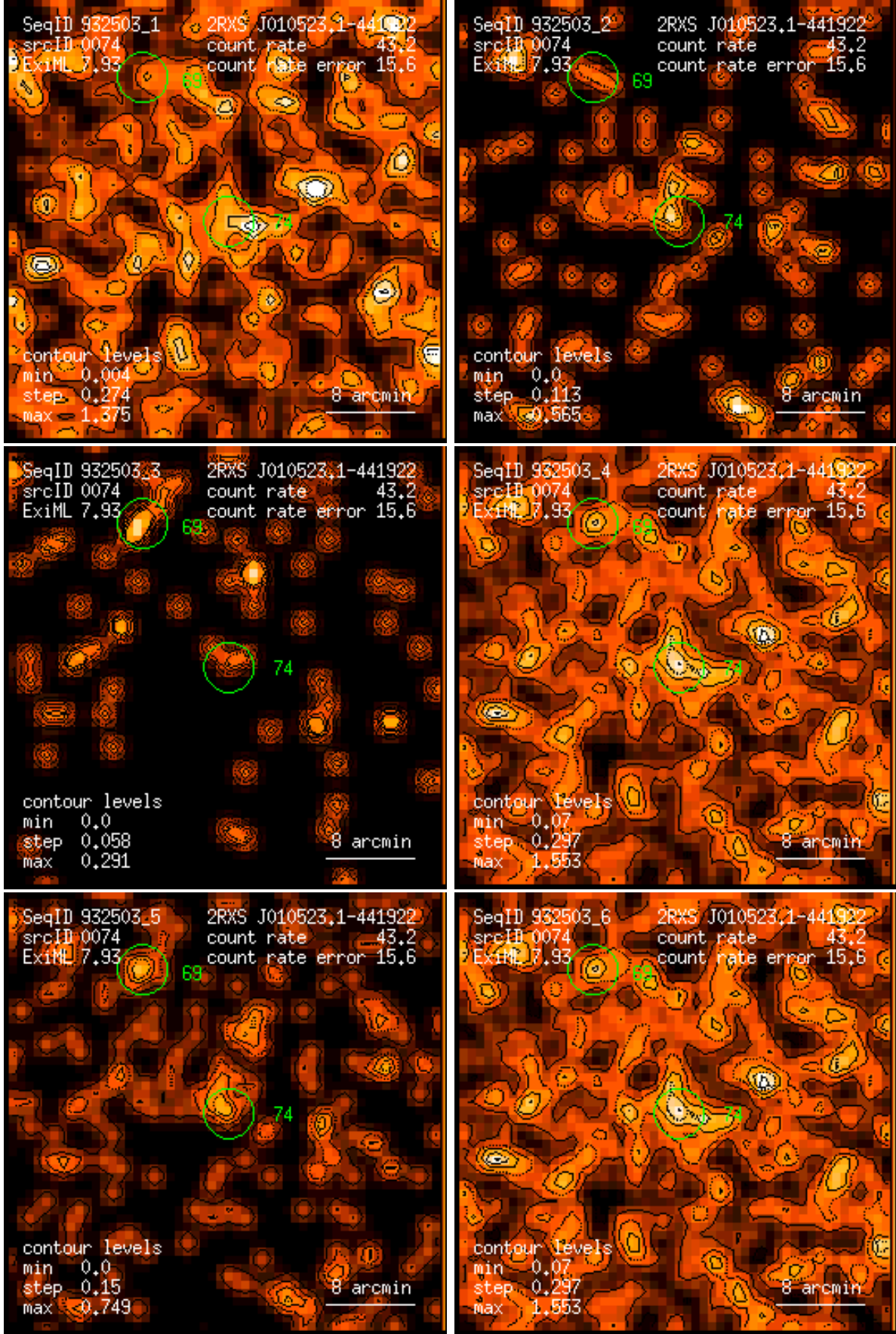
Figure 74: RASS 932503: detection 0074: band rate images, Gaussian filter: (1) PSPC channels 11 – 41, (2) 52 – 90, (3) 91 – 201, (4) 11 – 235, (5) 52 – 201, (6) 11 – 201. Broad band rates in counts/ks. Band rate contour levels in counts/ks/arcmin 2 .
