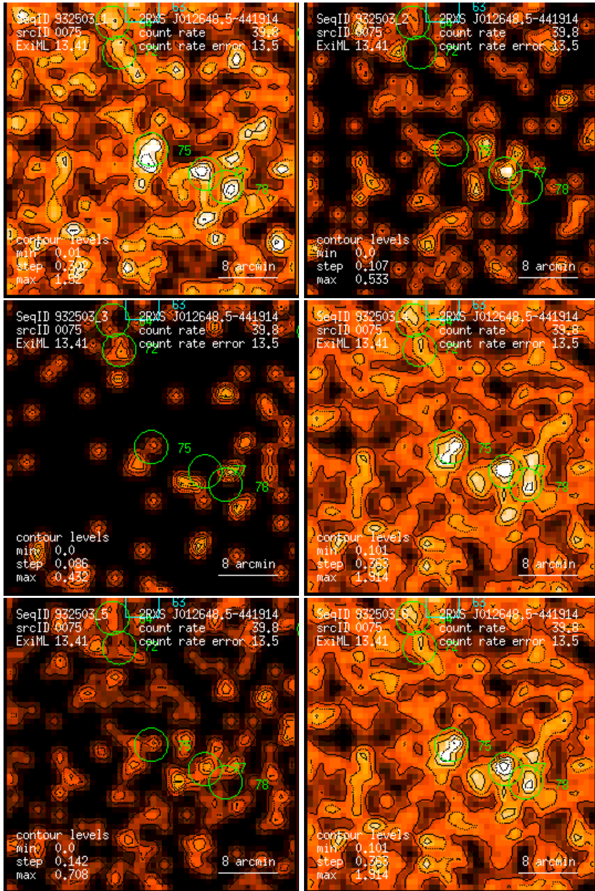
Figure 75: RASS 932503: detection 0075: band rate images, Gaussian filter: (1) PSPC channels 11 – 41, (2) 52 – 90, (3) 91 – 201, (4) 11 – 235, (5) 52 – 201, (6) 11 – 201. Broad band rates in counts/ks. Band rate contour levels in counts/ks/arcmin 2 .
