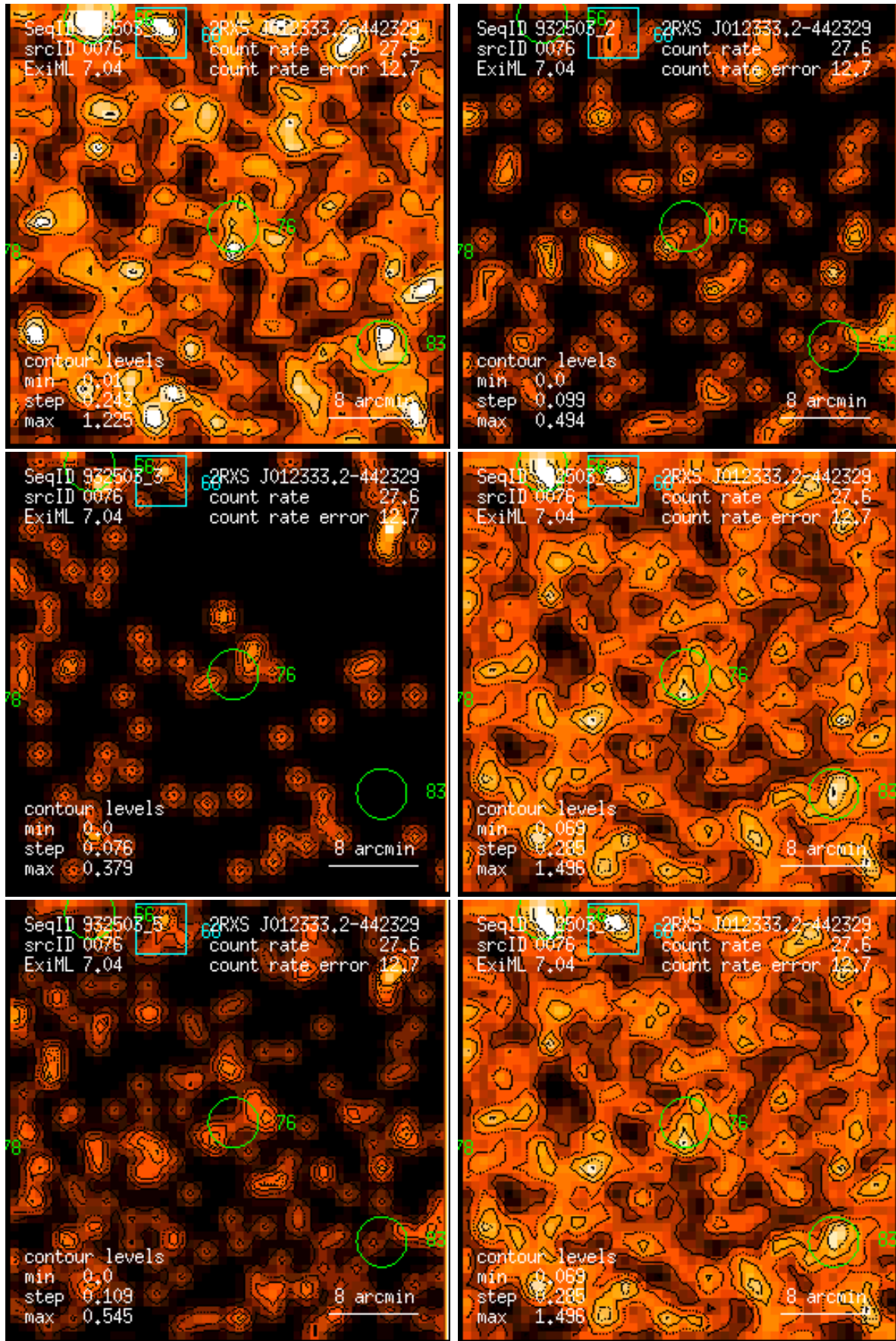
Figure 76: RASS 932503: detection 0076: band rate images, Gaussian filter: (1) PSPC channels 11 – 41, (2) 52 – 90, (3) 91 – 201, (4) 11 – 235, (5) 52 – 201, (6) 11 – 201. Broad band rates in counts/ks. Band rate contour levels in counts/ks/arcmin 2 .
