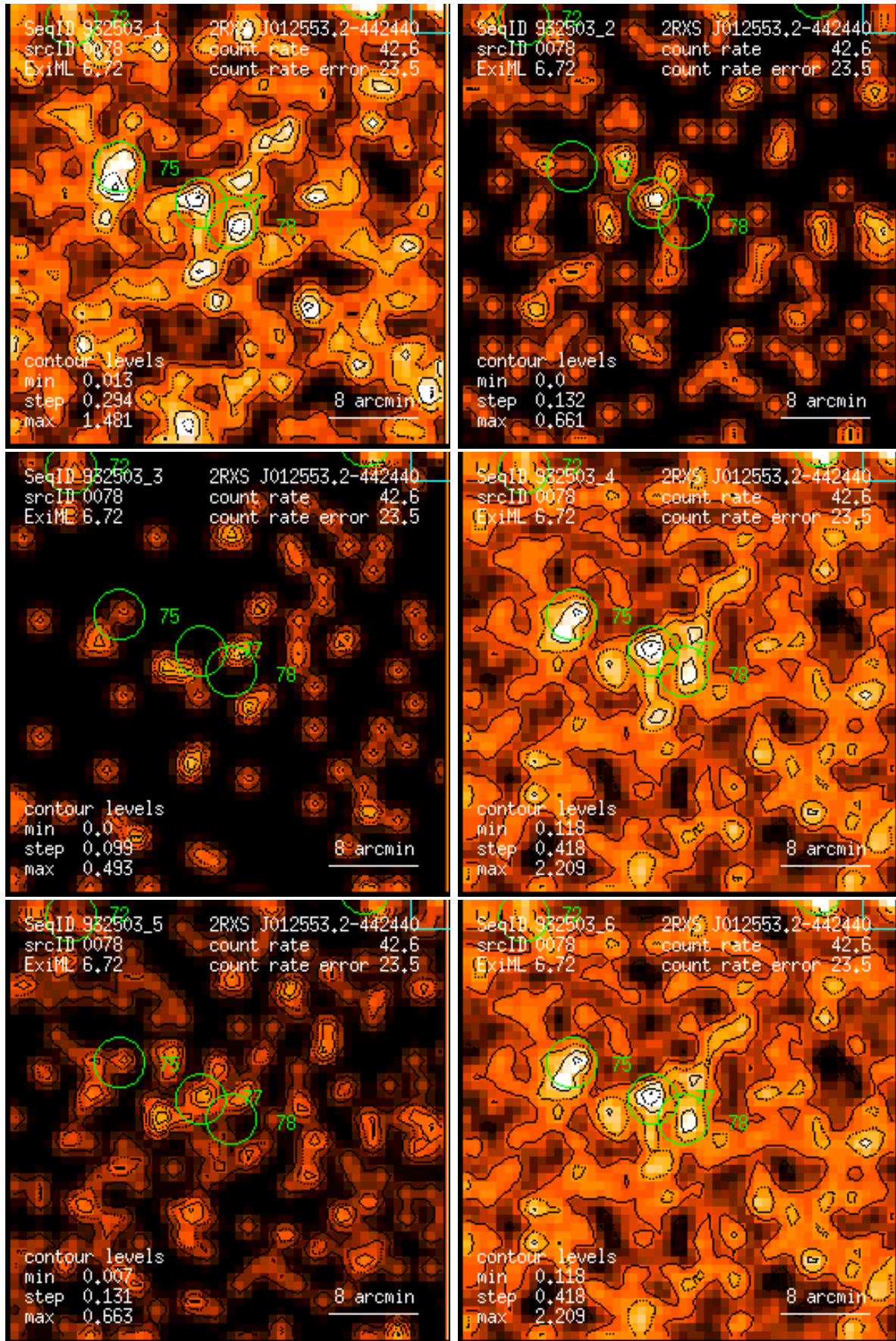
Figure 78: RASS 932503: detection 0078: band rate images, Gaussian filter: (1) PSPC channels 11 – 41, (2) 52 – 90, (3) 91 – 201, (4) 11 – 235, (5) 52 – 201, (6) 11 – 201. Broad band rates in counts/ks. Band rate contour levels in counts/ks/arcmin 2 .
