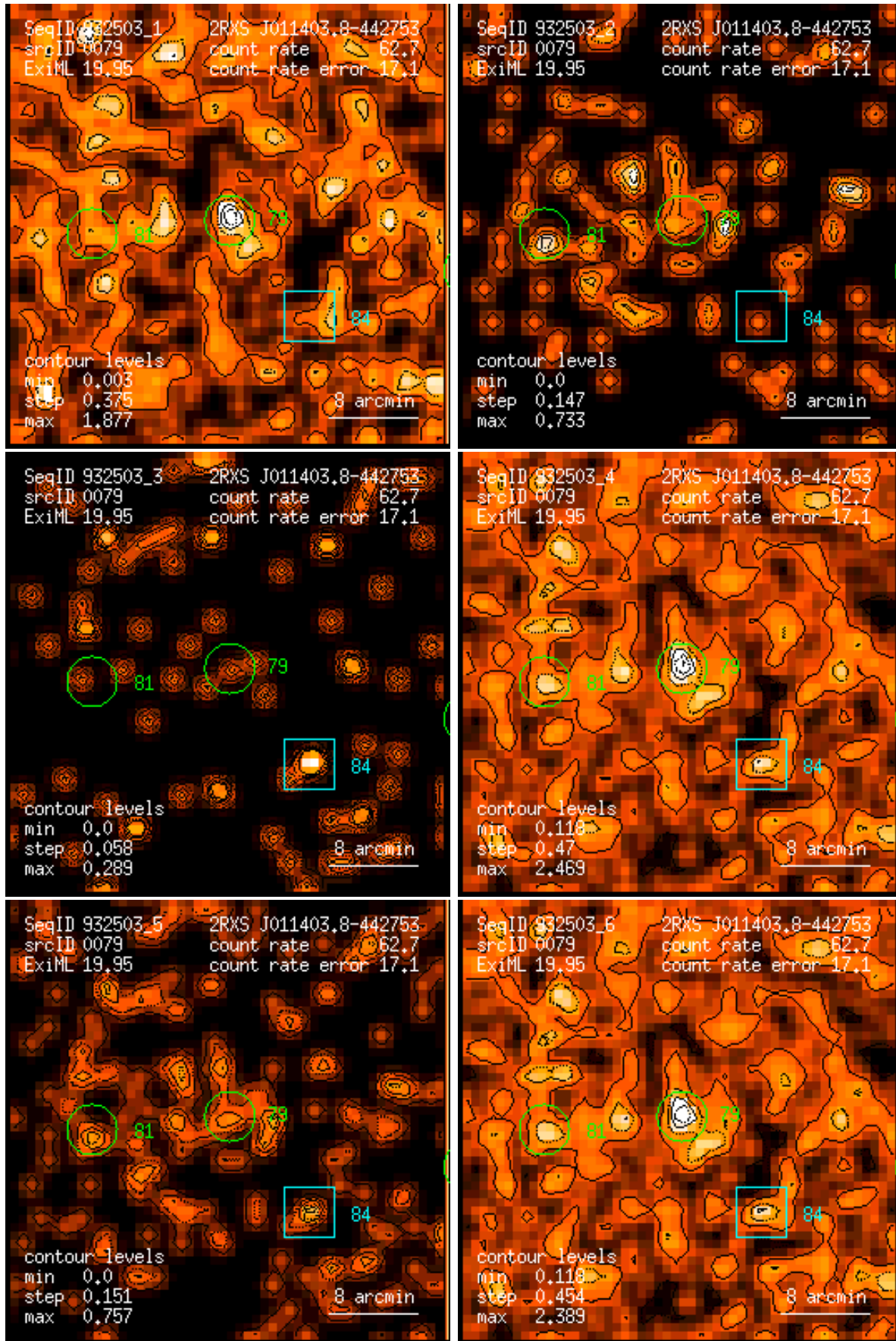
Figure 79: RASS 932503: detection 0079: band rate images, Gaussian filter: (1) PSPC channels 11 – 41, (2) 52 – 90, (3) 91 – 201, (4) 11 – 235, (5) 52 – 201, (6) 11 – 201. Broad band rates in counts/ks. Band rate contour levels in counts/ks/arcmin 2 .
