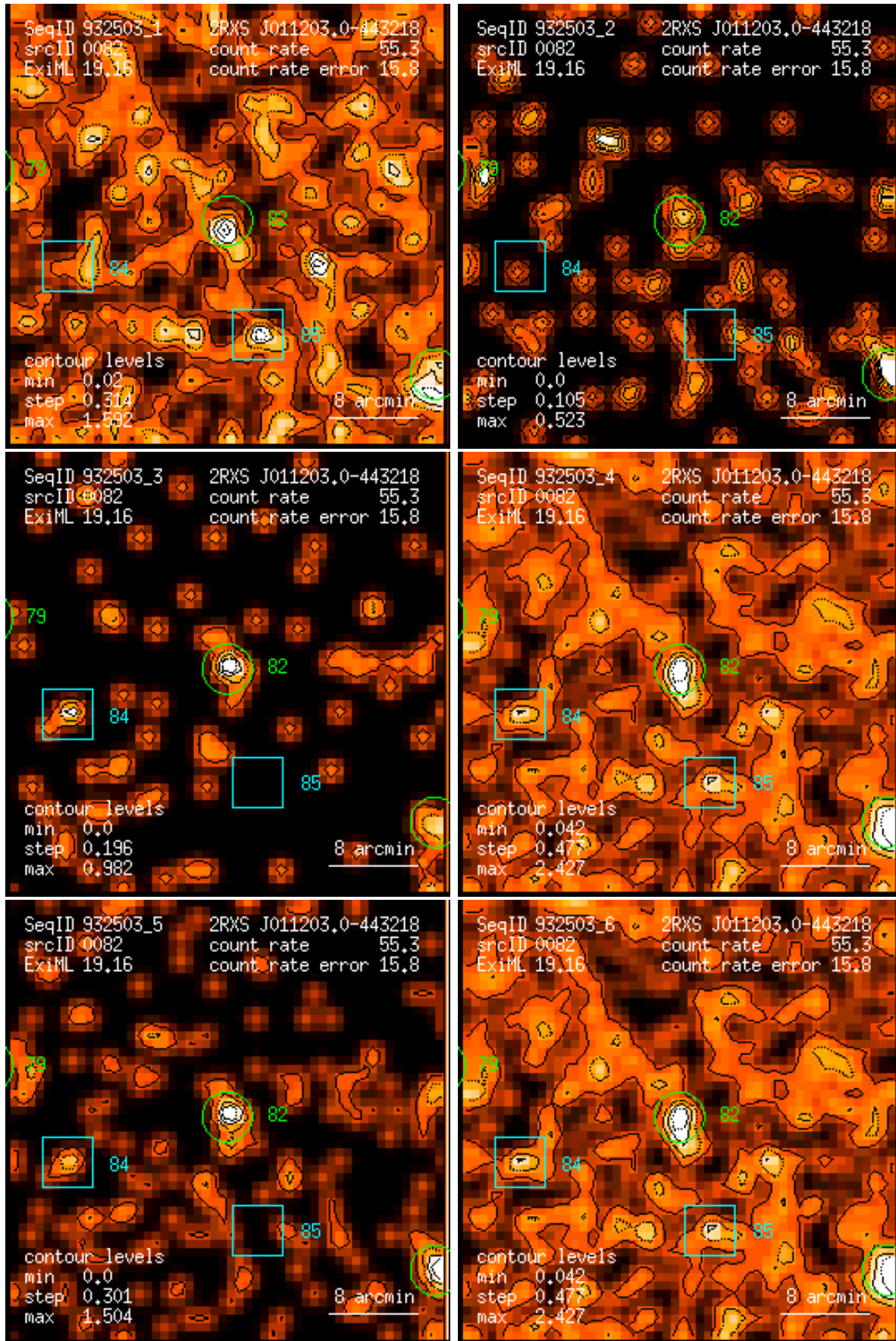
Figure 82: RASS 932503: detection 0082: band rate images, Gaussian filter: (1) PSPC channels 11 – 41, (2) 52 – 90, (3) 91 – 201, (4) 11 – 235, (5) 52 – 201, (6) 11 – 201. Broad band rates in counts/ks. Band rate contour levels in counts/ks/arcmin 2 .
