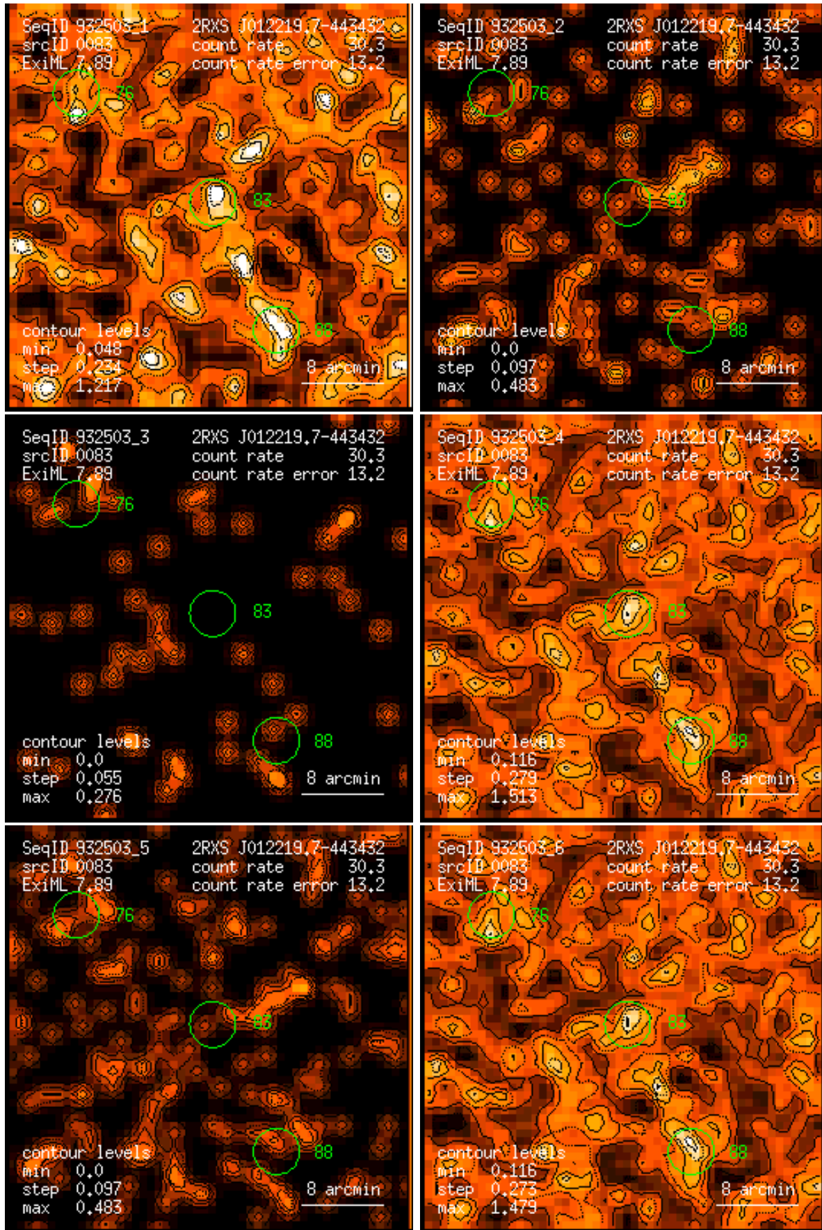
Figure 83: RASS 932503: detection 0083: band rate images, Gaussian filter: (1) PSPC channels 11 – 41, (2) 52 – 90, (3) 91 – 201, (4) 11 – 235, (5) 52 – 201, (6) 11 – 201. Broad band rates in counts/ks. Band rate contour levels in counts/ks/arcmin 2 .
