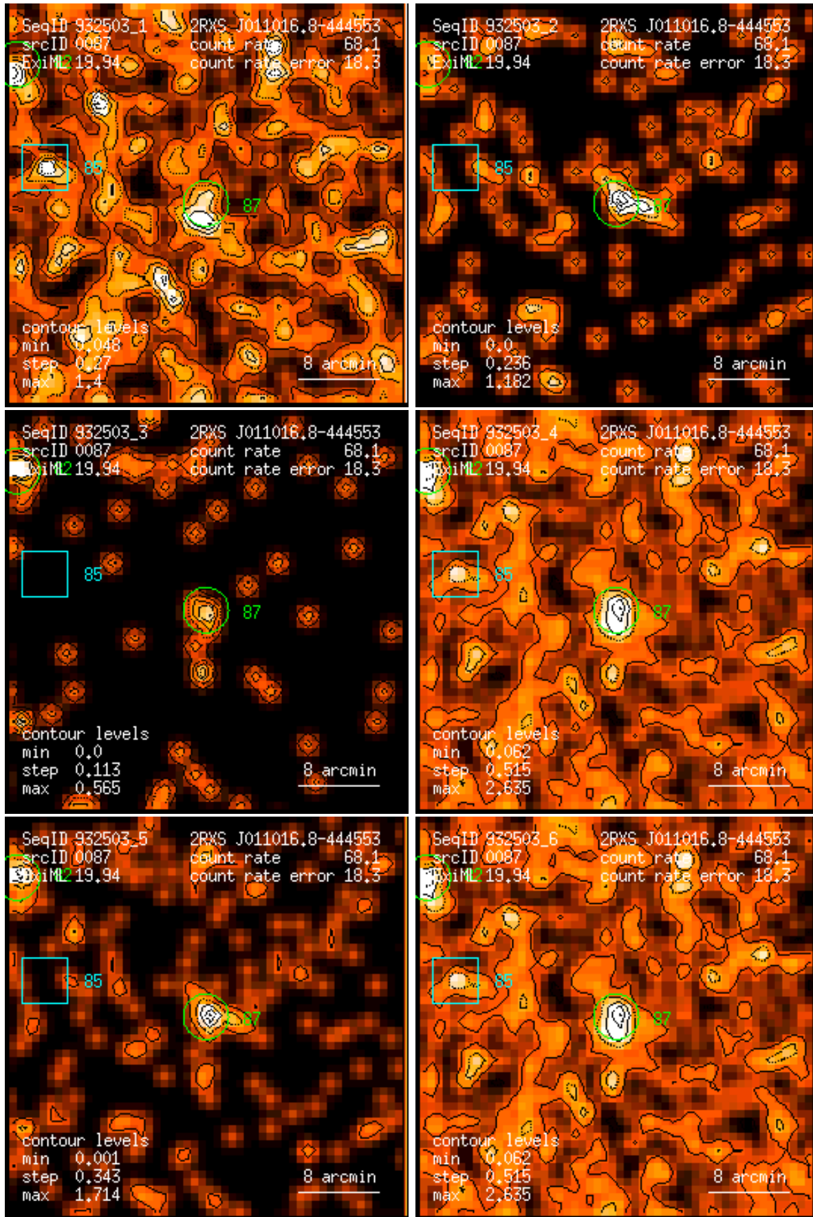
Figure 87: RASS 932503: detection 0087: band rate images, Gaussian filter: (1) PSPC channels 11 – 41, (2) 52 – 90, (3) 91 – 201, (4) 11 – 235, (5) 52 – 201, (6) 11 – 201. Broad band rates in counts/ks. Band rate contour levels in counts/ks/arcmin 2 .
