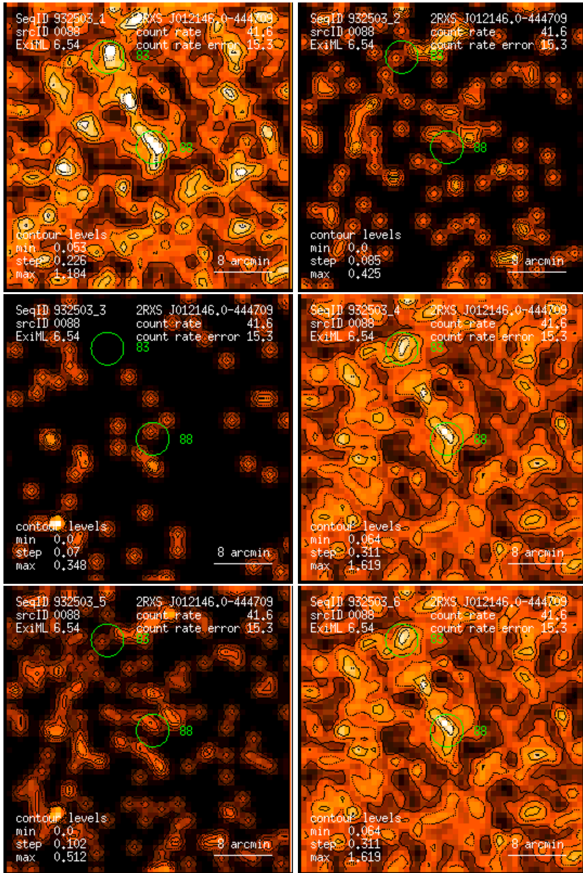
Figure 88: RASS 932503: detection 0088: band rate images, Gaussian filter: (1) PSPC channels 11 – 41, (2) 52 – 90, (3) 91 – 201, (4) 11 – 235, (5) 52 – 201, (6) 11 – 201. Broad band rates in counts/ks. Band rate contour levels in counts/ks/arcmin 2 .
