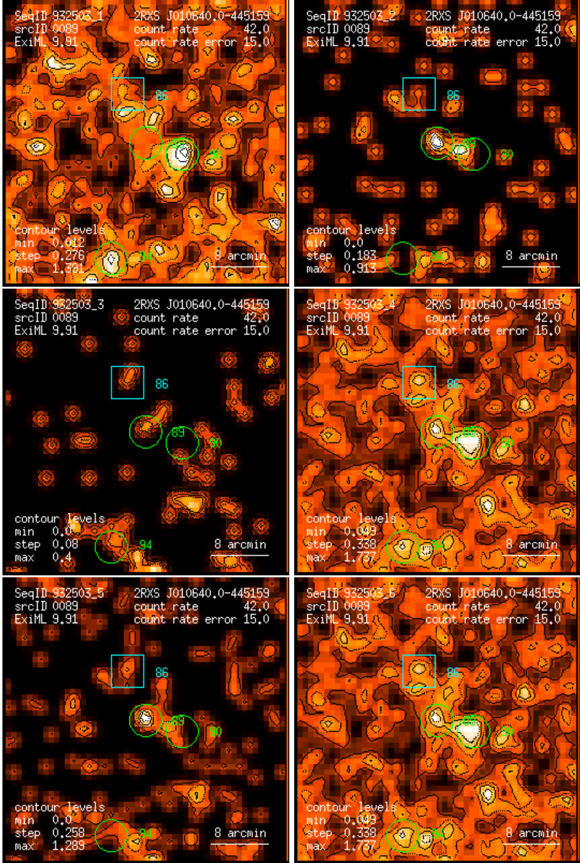
Figure 89: RASS 932503: detection 0089: band rate images, Gaussian filter: (1) PSPC channels 11 – 41, (2) 52 – 90, (3) 91 – 201, (4) 11 – 235, (5) 52 – 201, (6) 11 – 201. Broad band rates in counts/ks. Band rate contour levels in counts/ks/arcmin 2 .
