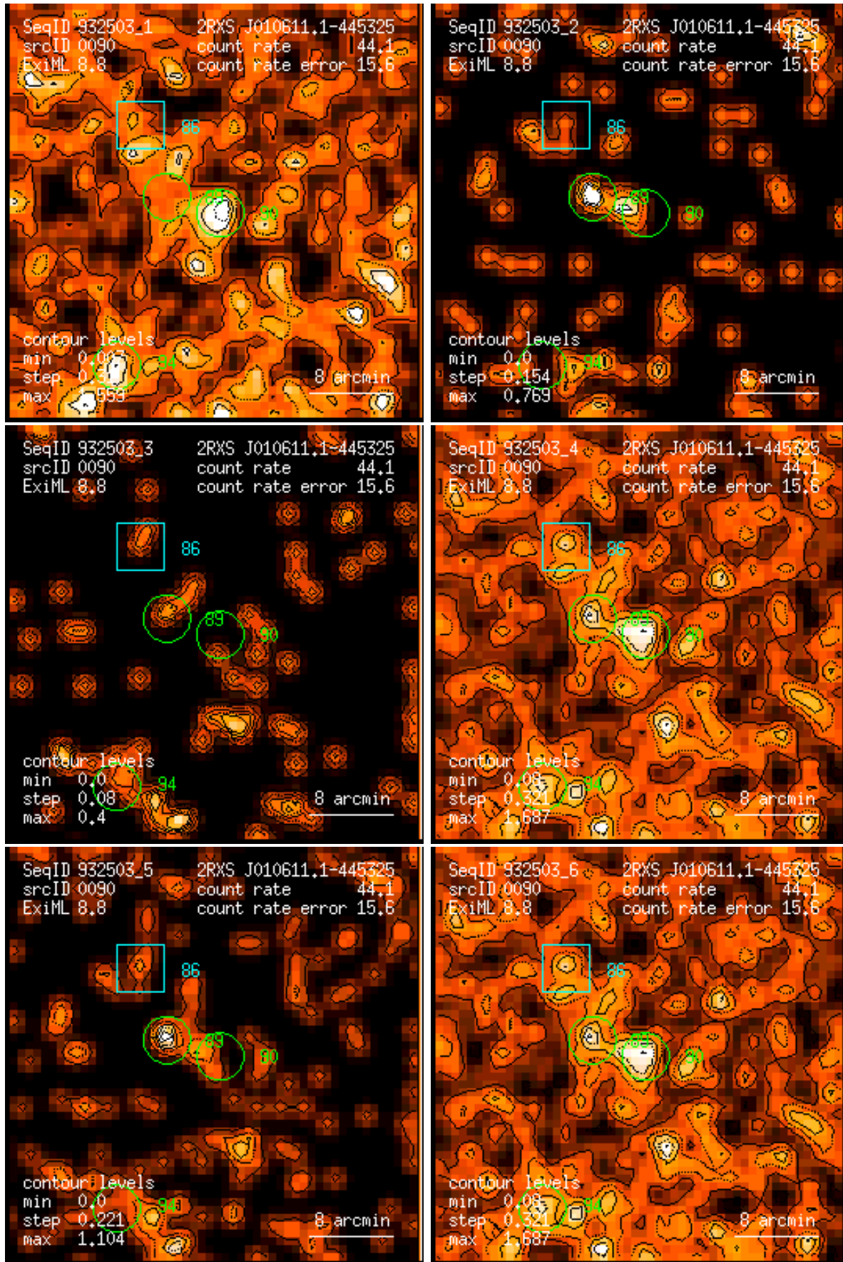
Figure 90: RASS 932503: detection 0090: band rate images, Gaussian filter: (1) PSPC channels 11 – 41, (2) 52 – 90, (3) 91 – 201, (4) 11 – 235, (5) 52 – 201, (6) 11 – 201. Broad band rates in counts/ks. Band rate contour levels in counts/ks/arcmin 2 .
