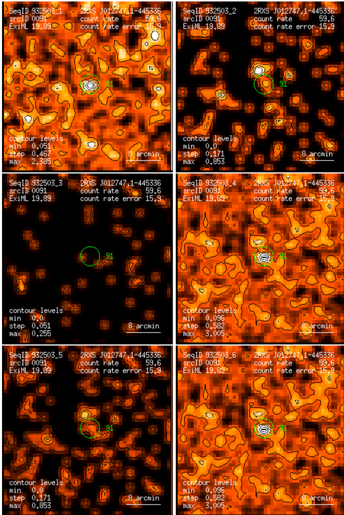
Figure 91: RASS 932503: detection 0091: band rate images, Gaussian filter: (1) PSPC channels 11 – 41, (2) 52 – 90, (3) 91 – 201, (4) 11 – 235, (5) 52 – 201, (6) 11 – 201. Broad band rates in counts/ks. Band rate contour levels in counts/ks/arcmin 2 .
