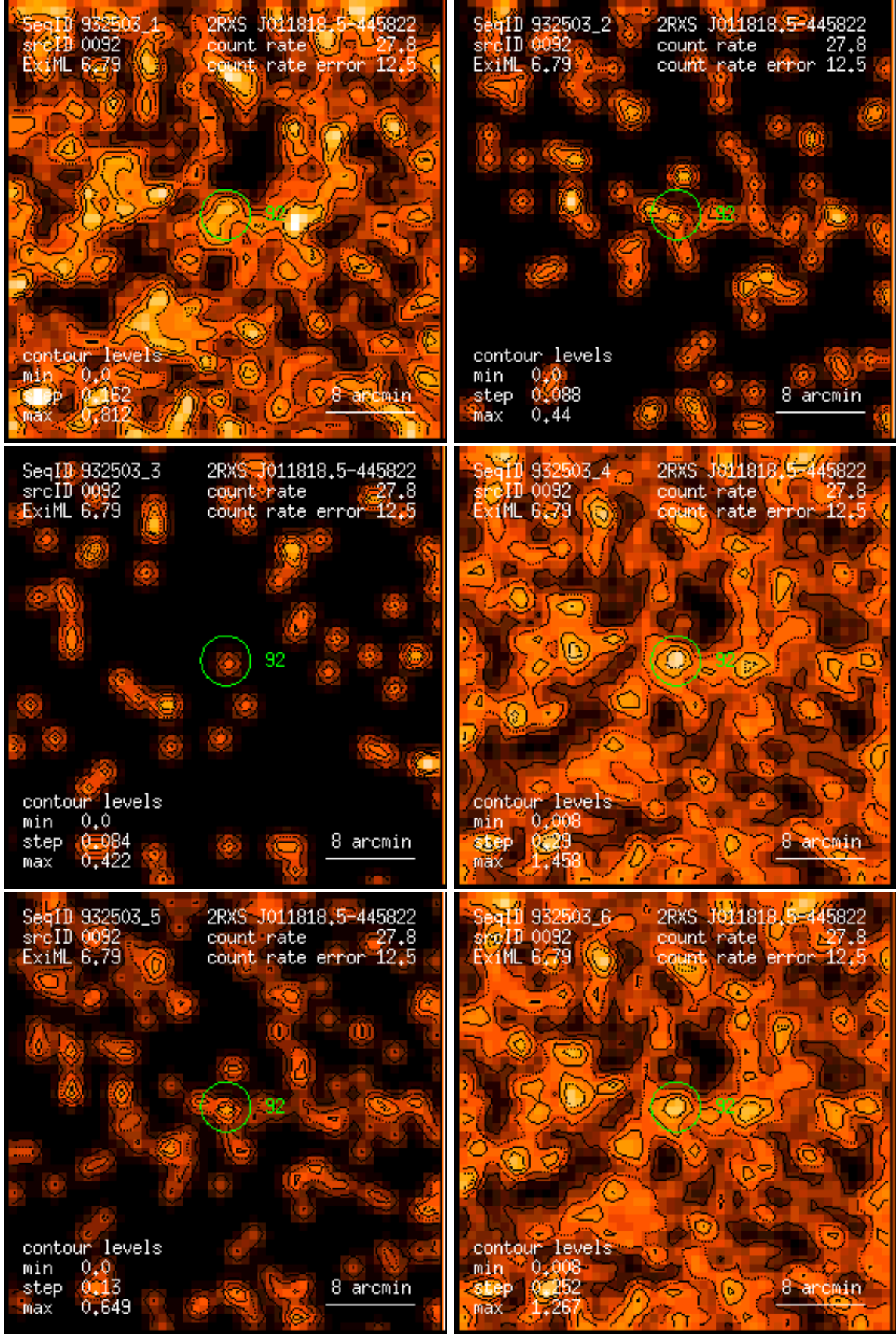
Figure 92: RASS 932503: detection 0092: band rate images, Gaussian filter: (1) PSPC channels 11 – 41, (2) 52 – 90, (3) 91 – 201, (4) 11 – 235, (5) 52 – 201, (6) 11 – 201. Broad band rates in counts/ks. Band rate contour levels in counts/ks/arcmin 2 .
