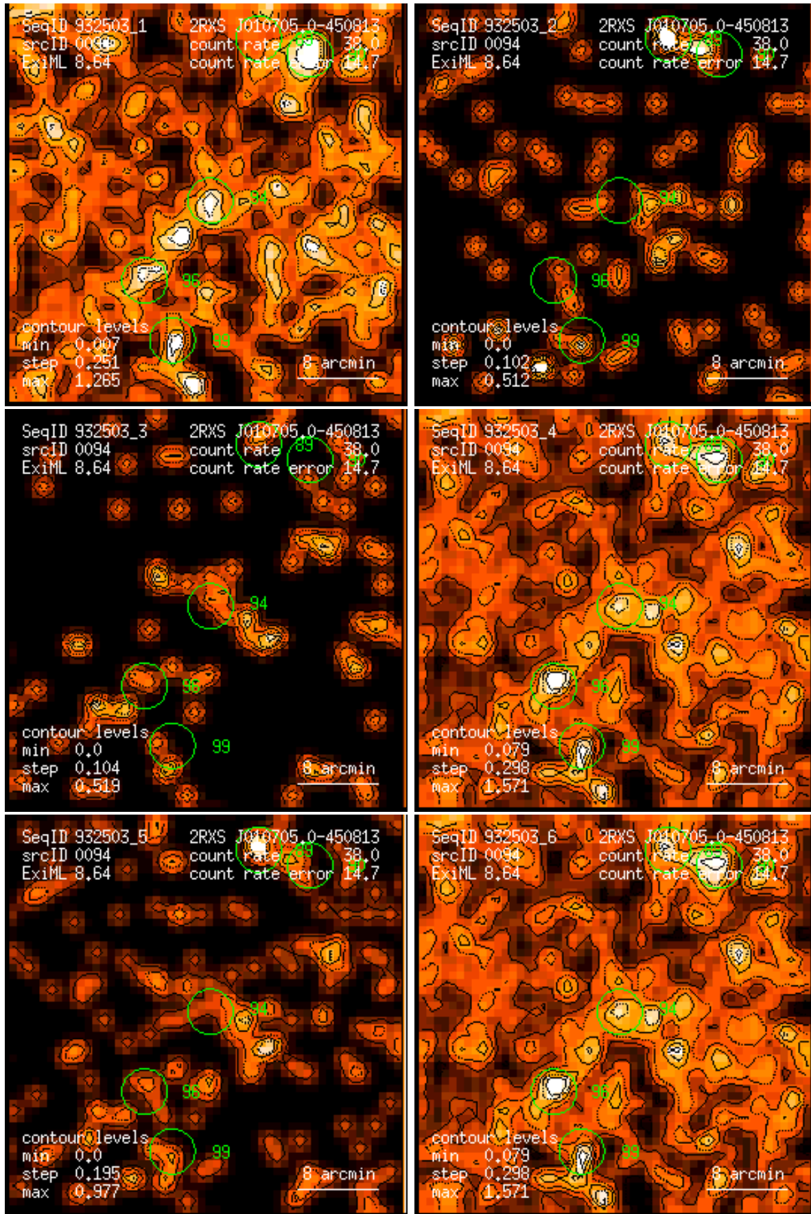
Figure 94: RASS 932503: detection 0094: band rate images, Gaussian filter: (1) PSPC channels 11 – 41, (2) 52 – 90, (3) 91 – 201, (4) 11 – 235, (5) 52 – 201, (6) 11 – 201. Broad band rates in counts/ks. Band rate contour levels in counts/ks/arcmin 2 .
