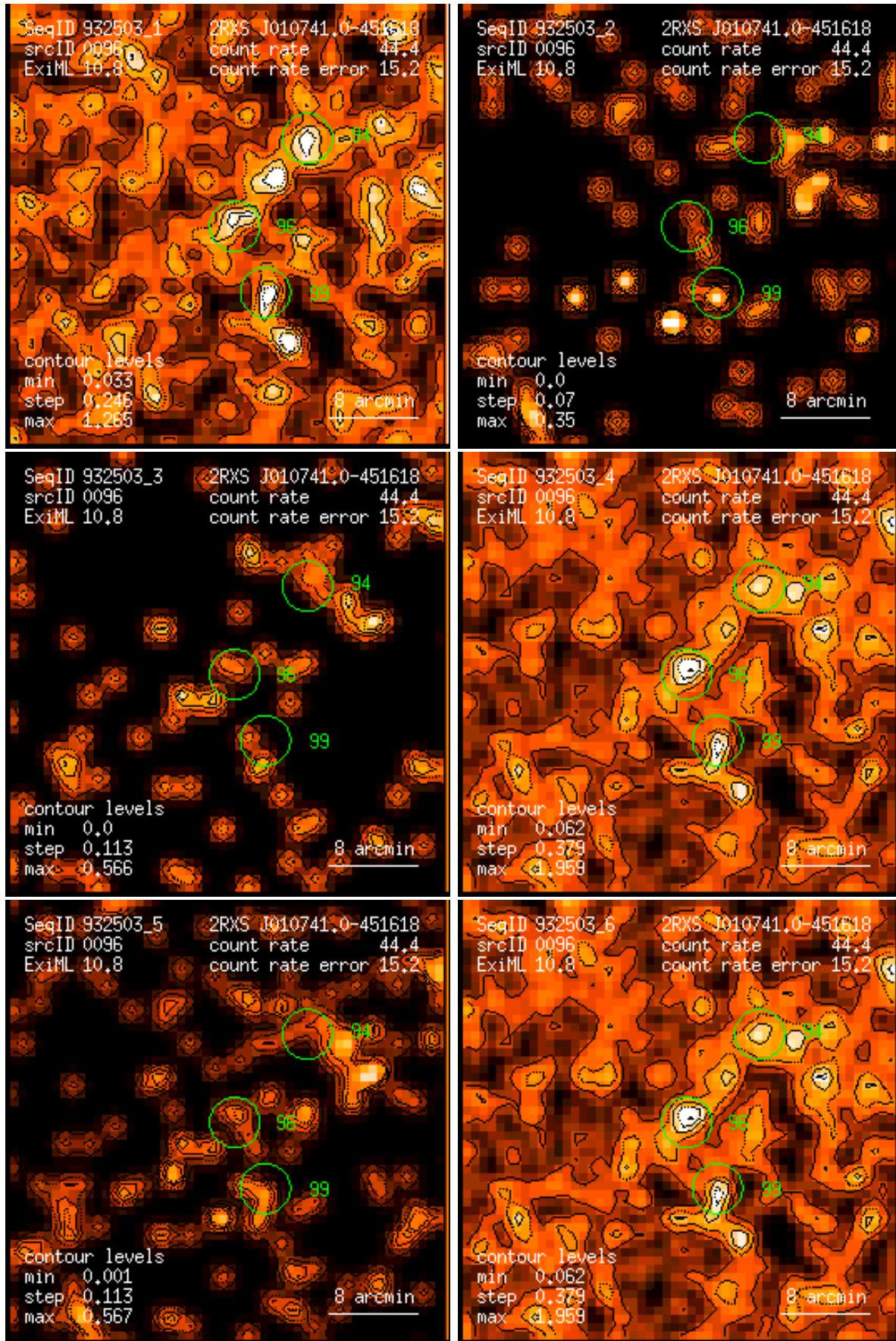
Figure 96: RASS 932503: detection 0096: band rate images, Gaussian filter: (1) PSPC channels 11 – 41, (2) 52 – 90, (3) 91 – 201, (4) 11 – 235, (5) 52 – 201, (6) 11 – 201. Broad band rates in counts/ks. Band rate contour levels in counts/ks/arcmin 2 .
