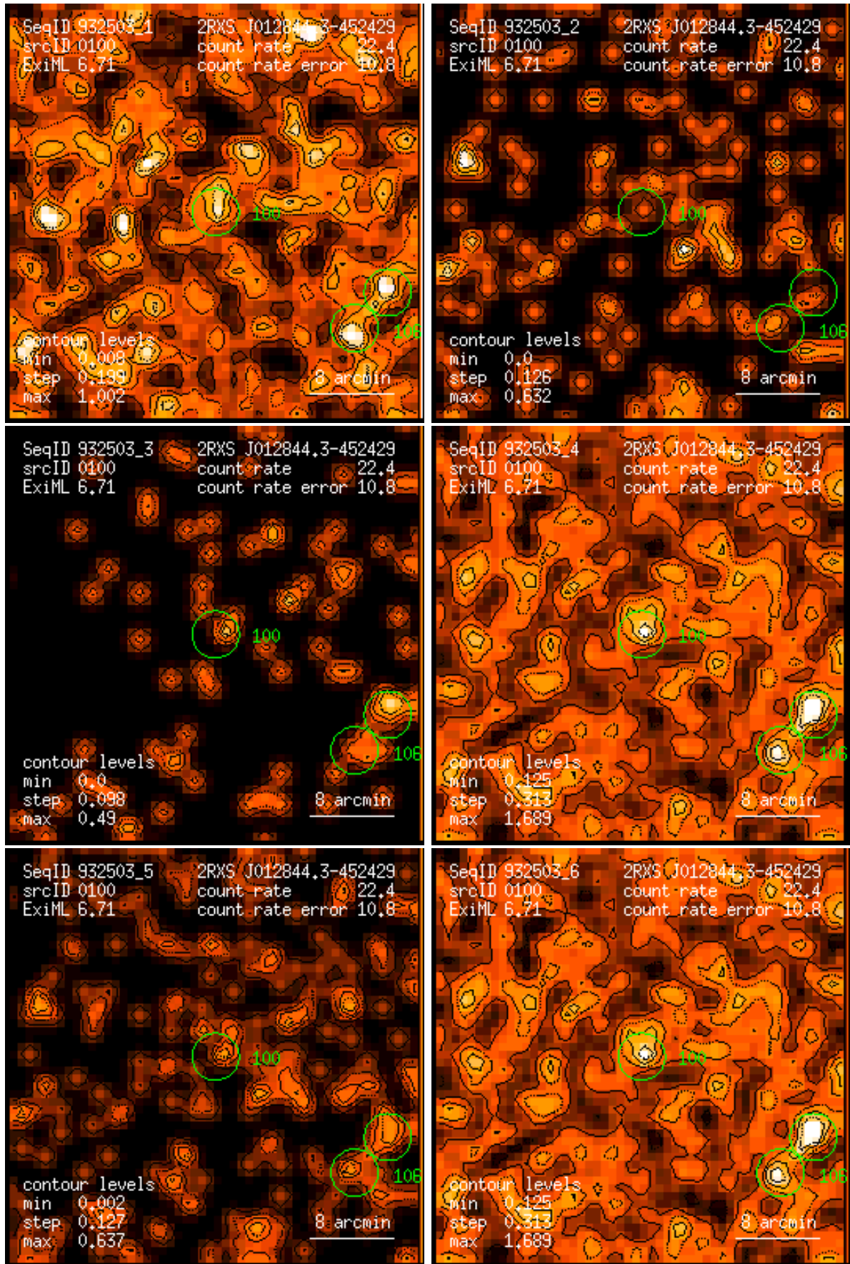
Figure 100: RASS 932503: detection 0100: band rate images, Gaussian filter: (1) PSPC channels 11 – 41, (2) 52 – 90, (3) 91 – 201, (4) 11 – 235, (5) 52 – 201, (6) 11 – 201. Broad band rates in counts/ks. Band rate contour levels in counts/ks/arcmin 2 .
