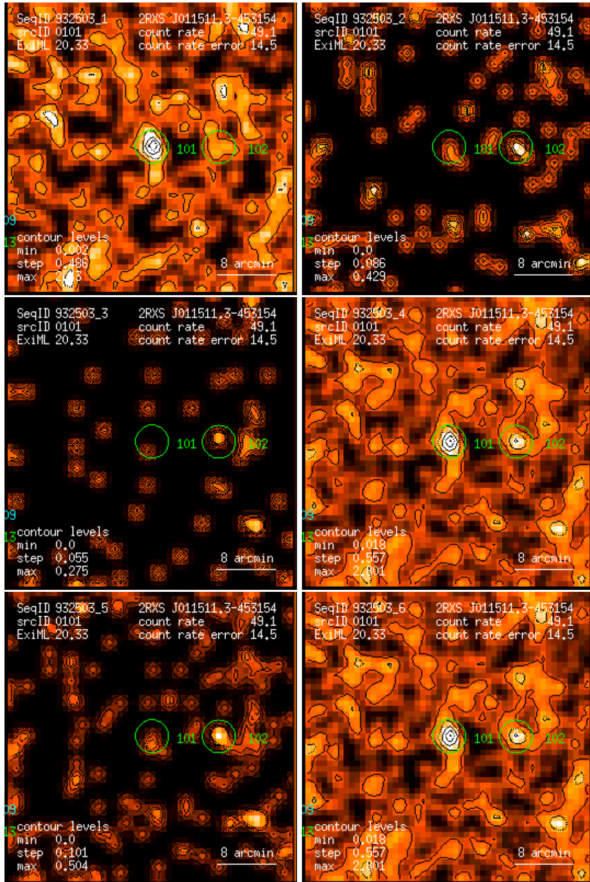
Figure 101: RASS 932503: detection 0101: band rate images, Gaussian filter: (1) PSPC channels 11 – 41, (2) 52 – 90, (3) 91 – 201, (4) 11 – 235, (5) 52 – 201, (6) 11 – 201. Broad band rates in counts/ks. Band rate contour levels in counts/ks/arcmin 2 .
