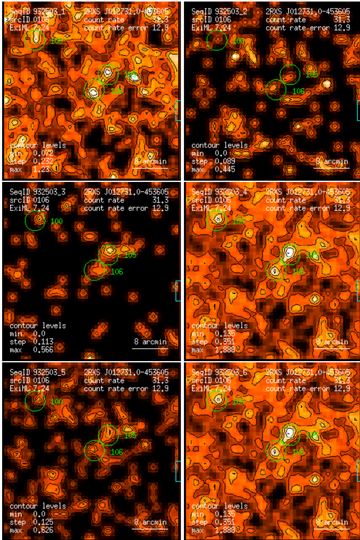
Figure 106: RASS 932503: detection 0106: band rate images, Gaussian filter: (1) PSPC channels 11 – 41, (2) 52 – 90, (3) 91 – 201, (4) 11 – 235, (5) 52 – 201, (6) 11 – 201. Broad band rates in counts/ks. Band rate contour levels in counts/ks/arcmin 2 .
