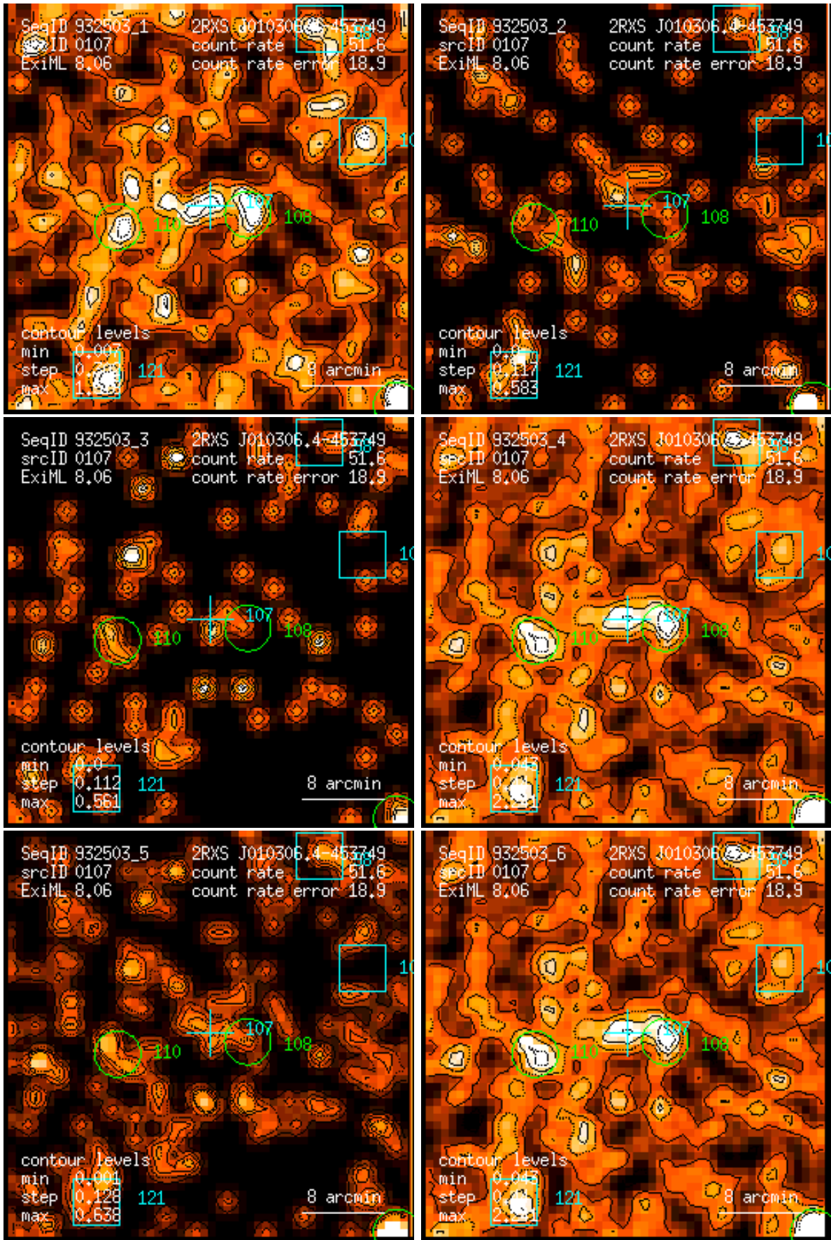
Figure 107: RASS 932503: detection 0107: band rate images, Gaussian filter: (1) PSPC channels 11 – 41, (2) 52 – 90, (3) 91 – 201, (4) 11 – 235, (5) 52 – 201, (6) 11 – 201. Broad band rates in counts/ks. Band rate contour levels in counts/ks/arcmin 2 .
