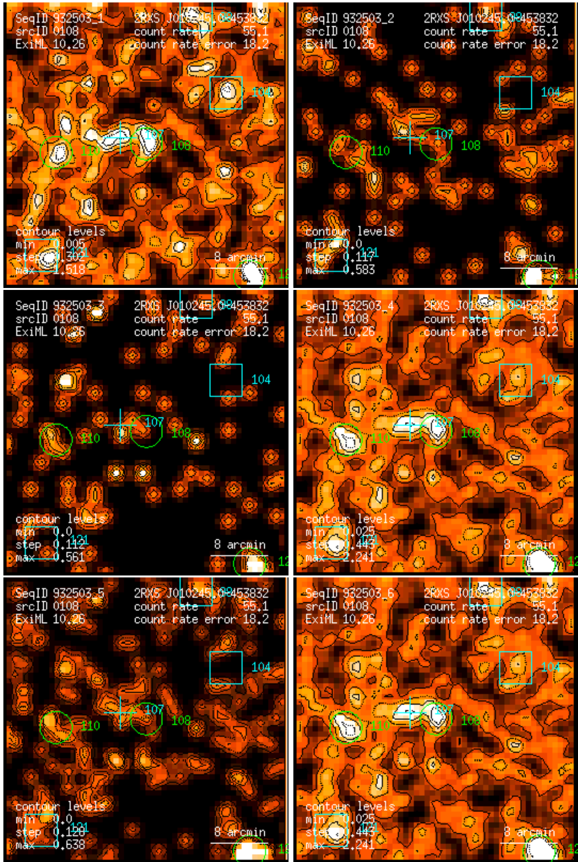
Figure 108: RASS 932503: detection 0108: band rate images, Gaussian filter: (1) PSPC channels 11 – 41, (2) 52 – 90, (3) 91 – 201, (4) 11 – 235, (5) 52 – 201, (6) 11 – 201. Broad band rates in counts/ks. Band rate contour levels in counts/ks/arcmin 2 .
