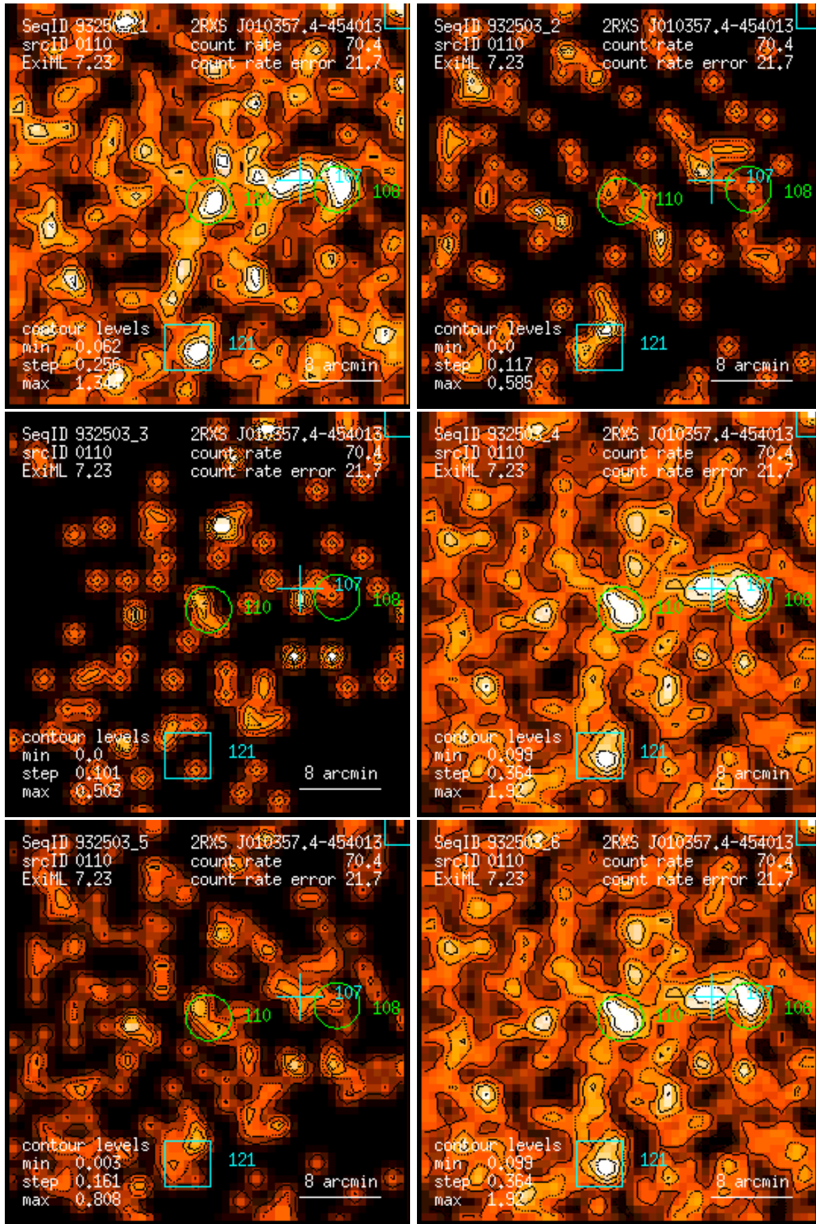
Figure 110: RASS 932503: detection 0110: band rate images, Gaussian filter: (1) PSPC channels 11 – 41, (2) 52 – 90, (3) 91 – 201, (4) 11 – 235, (5) 52 – 201, (6) 11 – 201. Broad band rates in counts/ks. Band rate contour levels in counts/ks/arcmin 2 .
