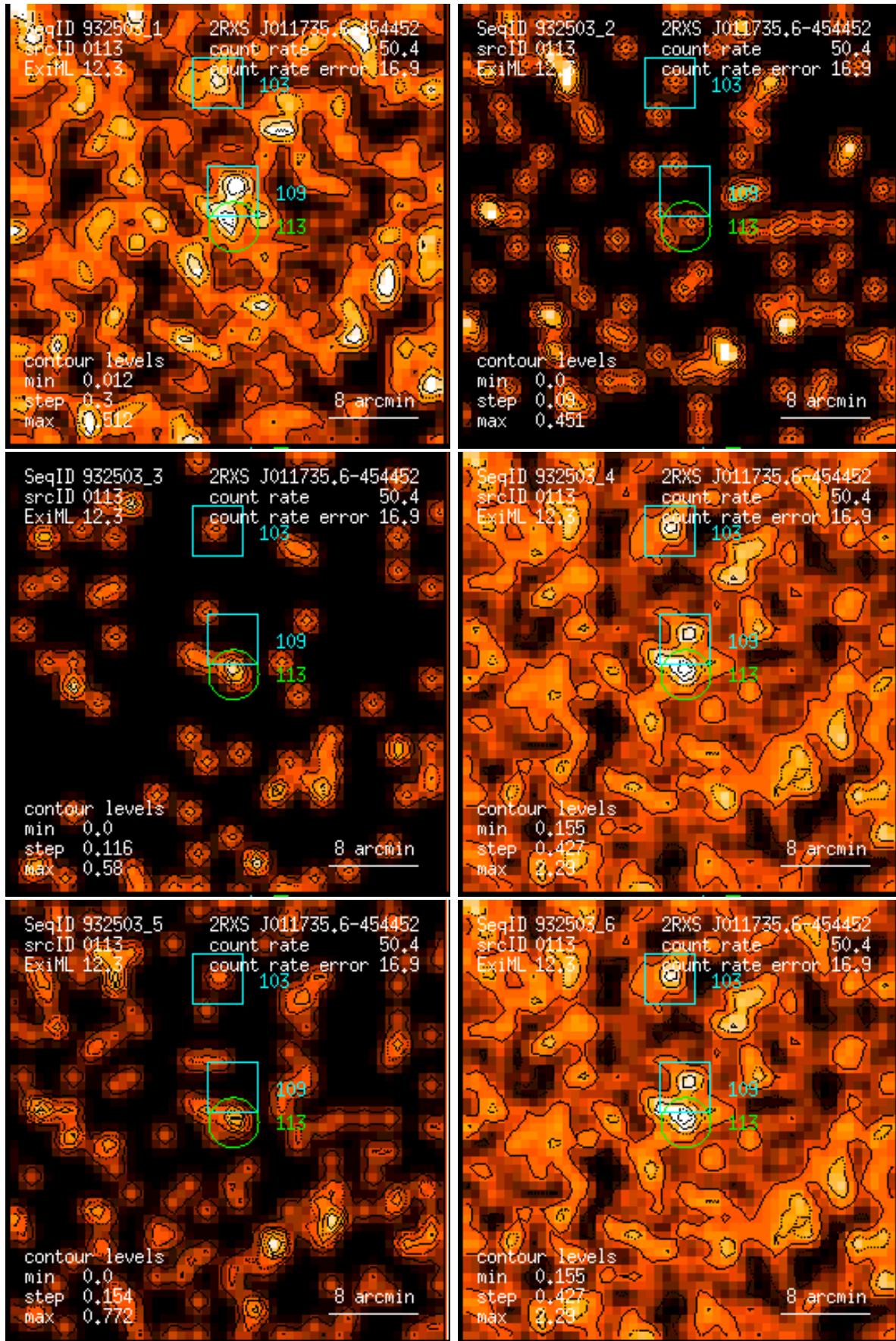
Figure 113: RASS 932503: detection 0113: band rate images, Gaussian filter: (1) PSPC channels 11 – 41, (2) 52 – 90, (3) 91 – 201, (4) 11 – 235, (5) 52 – 201, (6) 11 – 201. Broad band rates in counts/ks. Band rate contour levels in counts/ks/arcmin 2 .
