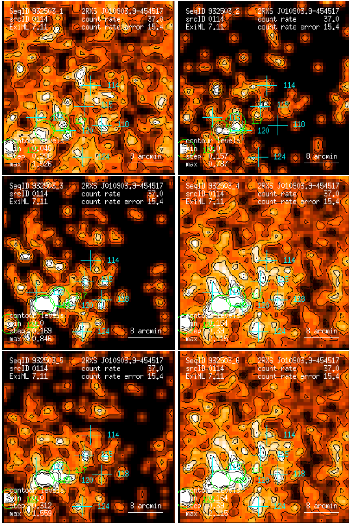
Figure 114: RASS 932503: detection 0114: band rate images, Gaussian filter: (1) PSPC channels 11 – 41, (2) 52 – 90, (3) 91 – 201, (4) 11 – 235, (5) 52 – 201, (6) 11 – 201. Broad band rates in counts/ks. Band rate contour levels in counts/ks/arcmin 2 .
