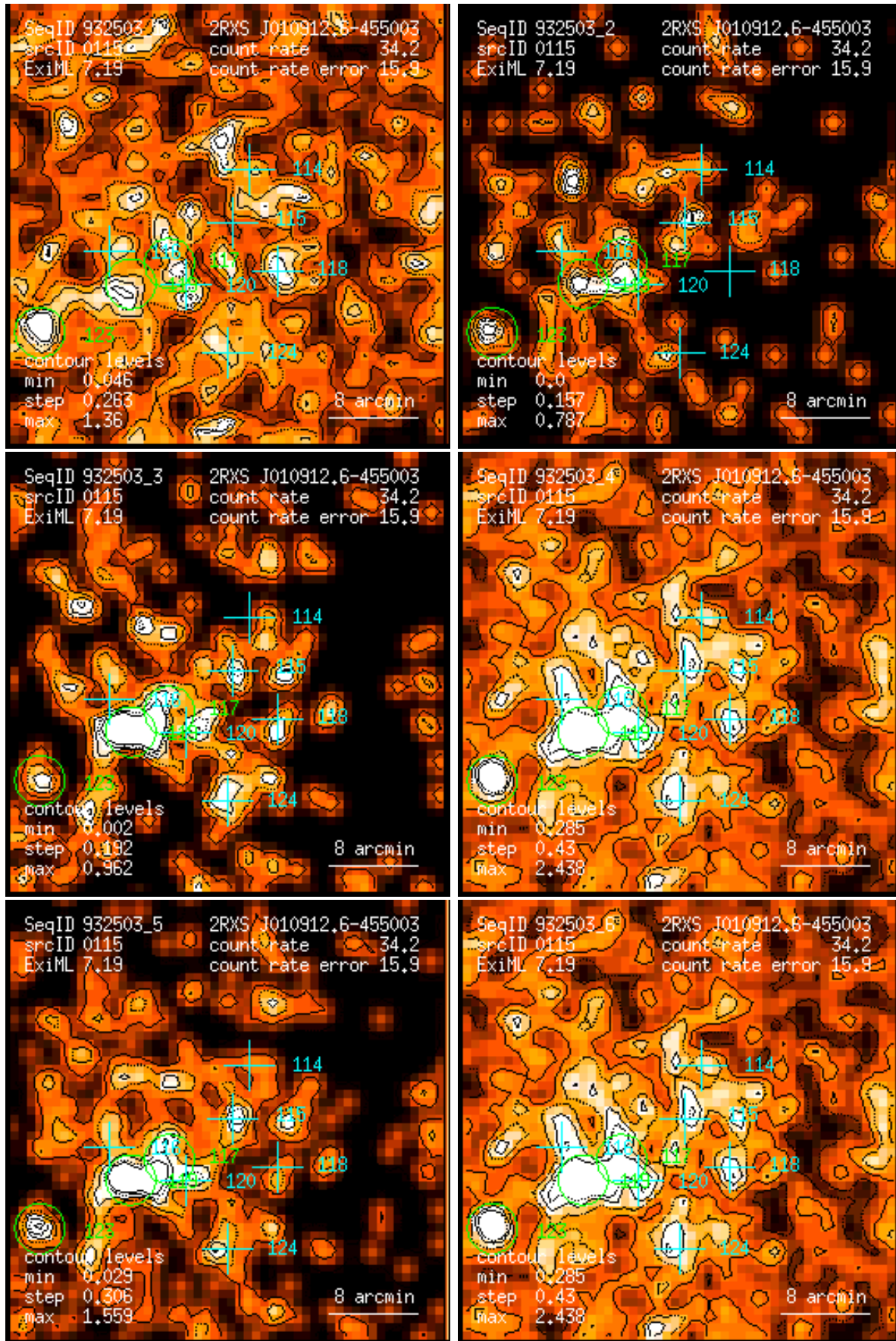
Figure 115: RASS 932503: detection 0115: band rate images, Gaussian filter: (1) PSPC channels 11 – 41, (2) 52 – 90, (3) 91 – 201, (4) 11 – 235, (5) 52 – 201, (6) 11 – 201. Broad band rates in counts/ks. Band rate contour levels in counts/ks/arcmin 2 .
