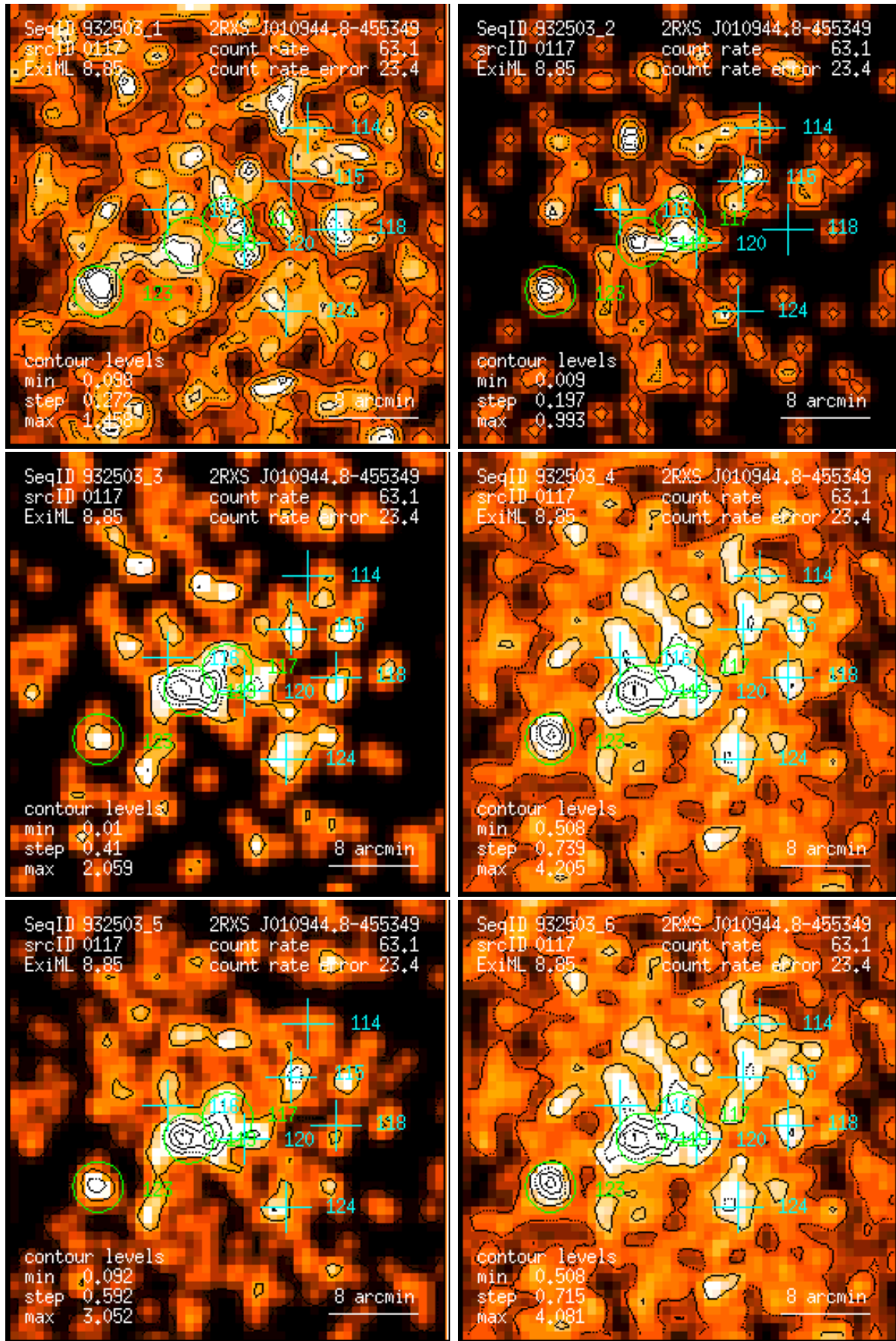
Figure 117: RASS 932503: detection 0117: band rate images, Gaussian filter: (1) PSPC channels 11 – 41, (2) 52 – 90, (3) 91 – 201, (4) 11 – 235, (5) 52 – 201, (6) 11 – 201. Broad band rates in counts/ks. Band rate contour levels in counts/ks/arcmin 2 .
