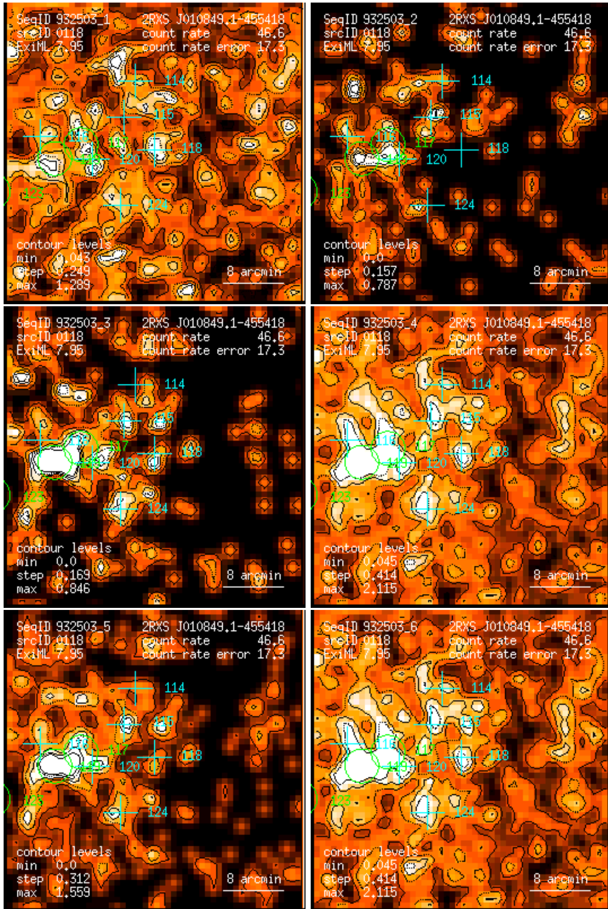
Figure 118: RASS 932503: detection 0118: band rate images, Gaussian filter: (1) PSPC channels 11 – 41, (2) 52 – 90, (3) 91 – 201, (4) 11 – 235, (5) 52 – 201, (6) 11 – 201. Broad band rates in counts/ks. Band rate contour levels in counts/ks/arcmin 2 .
