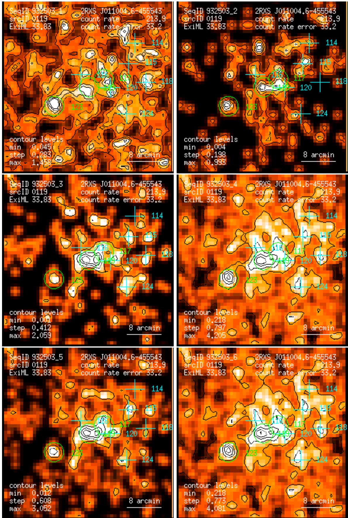
Figure 119: RASS 932503: detection 0119: band rate images, Gaussian filter: (1) PSPC channels 11 – 41, (2) 52 – 90, (3) 91 – 201, (4) 11 – 235, (5) 52 – 201, (6) 11 – 201. Broad band rates in counts/ks. Band rate contour levels in counts/ks/arcmin 2 .
