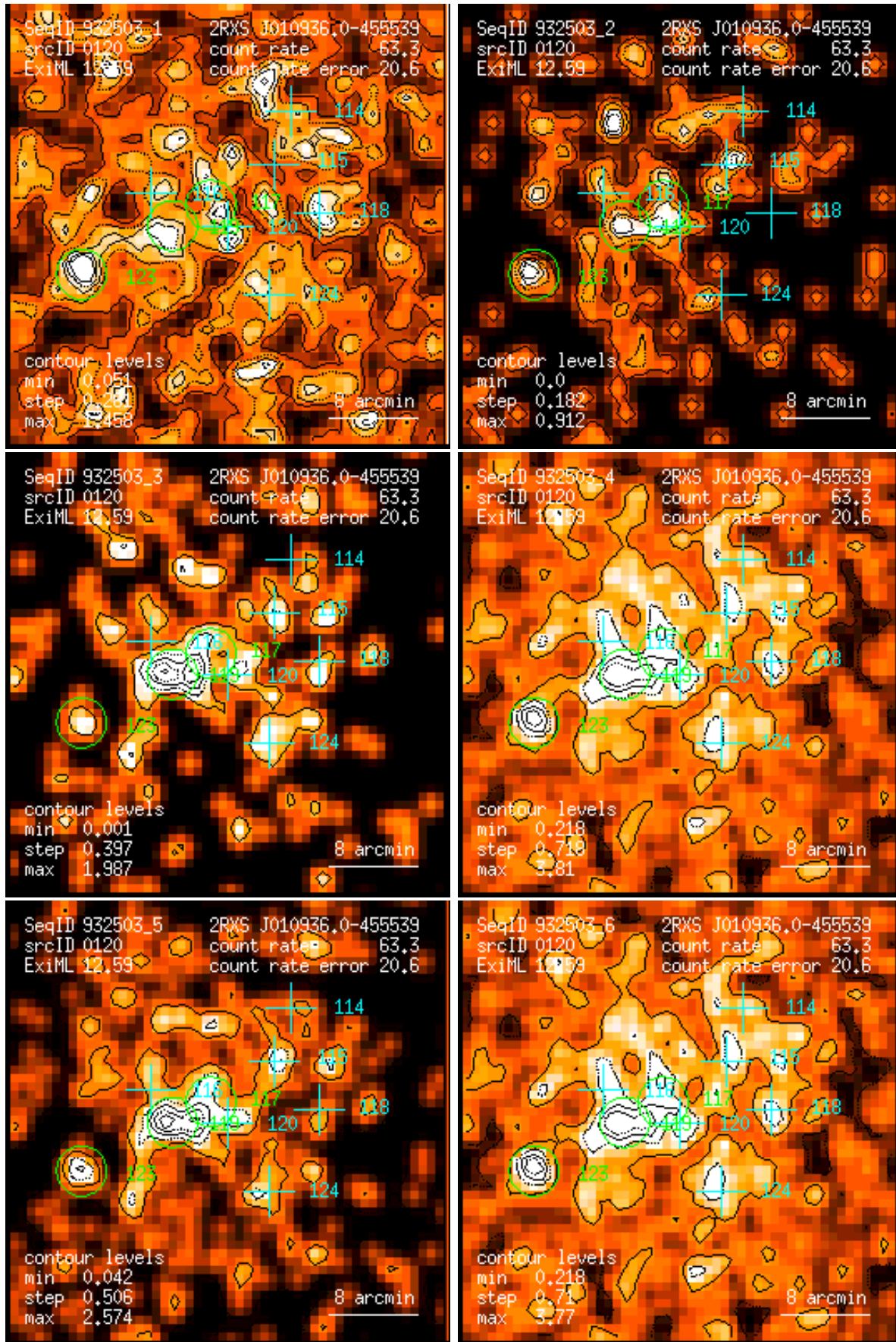
Figure 120: RASS 932503: detection 0120: band rate images, Gaussian filter: (1) PSPC channels 11 – 41, (2) 52 – 90, (3) 91 – 201, (4) 11 – 235, (5) 52 – 201, (6) 11 – 201. Broad band rates in counts/ks. Band rate contour levels in counts/ks/arcmin 2 .
