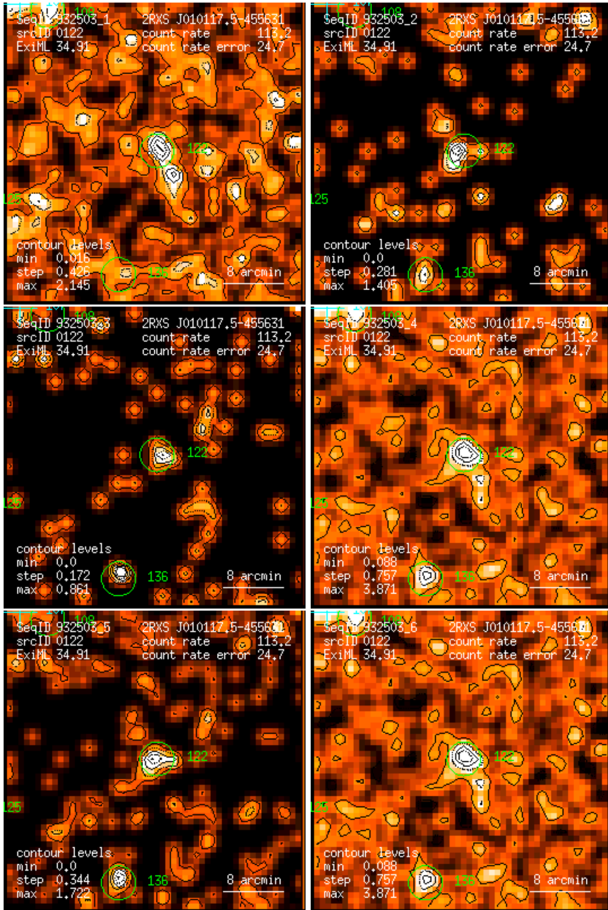
Figure 122: RASS 932503: detection 0122: band rate images, Gaussian filter: (1) PSPC channels 11 – 41, (2) 52 – 90, (3) 91 – 201, (4) 11 – 235, (5) 52 – 201, (6) 11 – 201. Broad band rates in counts/ks. Band rate contour levels in counts/ks/arcmin 2 .
