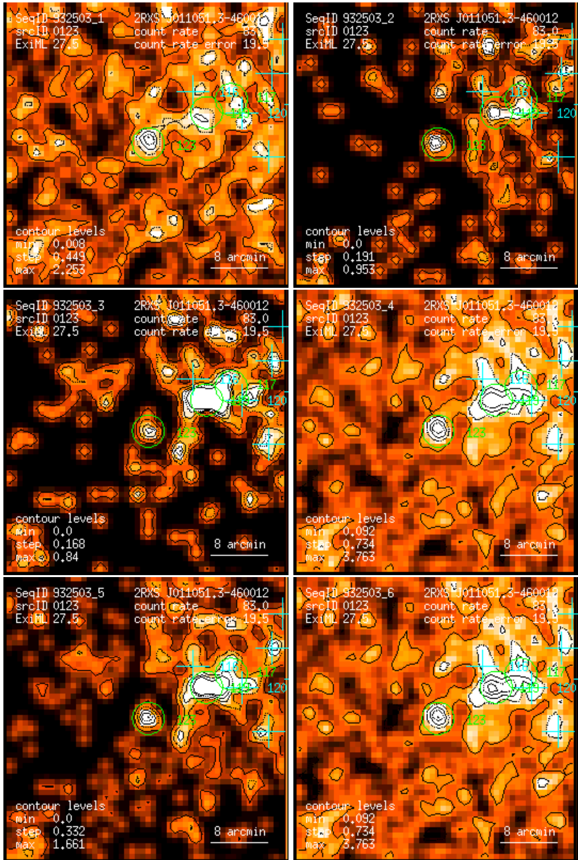
Figure 123: RASS 932503: detection 0123: band rate images, Gaussian filter: (1) PSPC channels 11 – 41, (2) 52 – 90, (3) 91 – 201, (4) 11 – 235, (5) 52 – 201, (6) 11 – 201. Broad band rates in counts/ks. Band rate contour levels in counts/ks/arcmin 2 .
