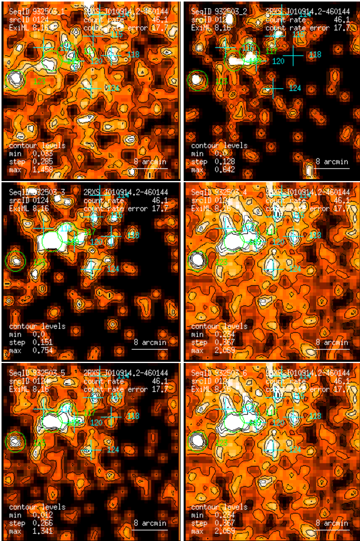
Figure 124: RASS 932503: detection 0124: band rate images, Gaussian filter: (1) PSPC channels 11 – 41, (2) 52 – 90, (3) 91 – 201, (4) 11 – 235, (5) 52 – 201, (6) 11 – 201. Broad band rates in counts/ks. Band rate contour levels in counts/ks/arcmin 2 .
