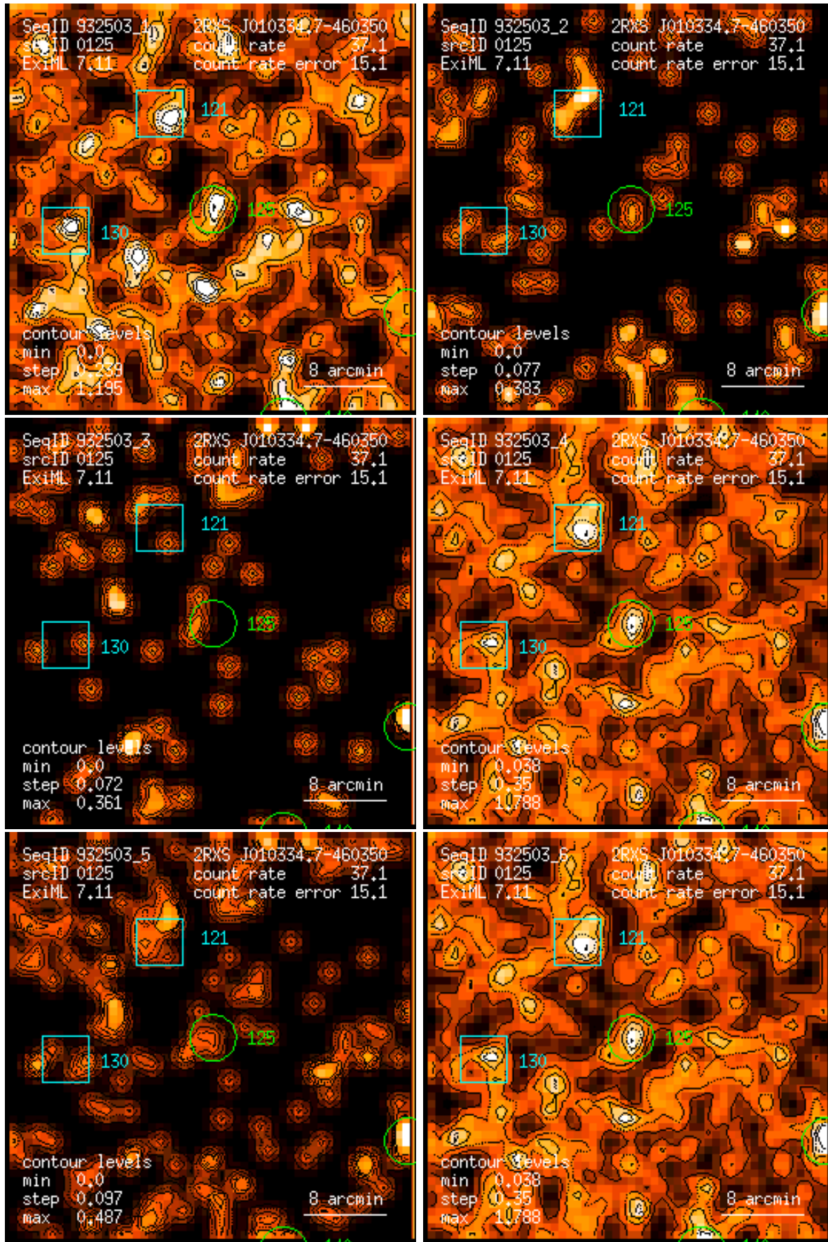
Figure 125: RASS 932503: detection 0125: band rate images, Gaussian filter: (1) PSPC channels 11 – 41, (2) 52 – 90, (3) 91 – 201, (4) 11 – 235, (5) 52 – 201, (6) 11 – 201. Broad band rates in counts/ks. Band rate contour levels in counts/ks/arcmin 2 .
