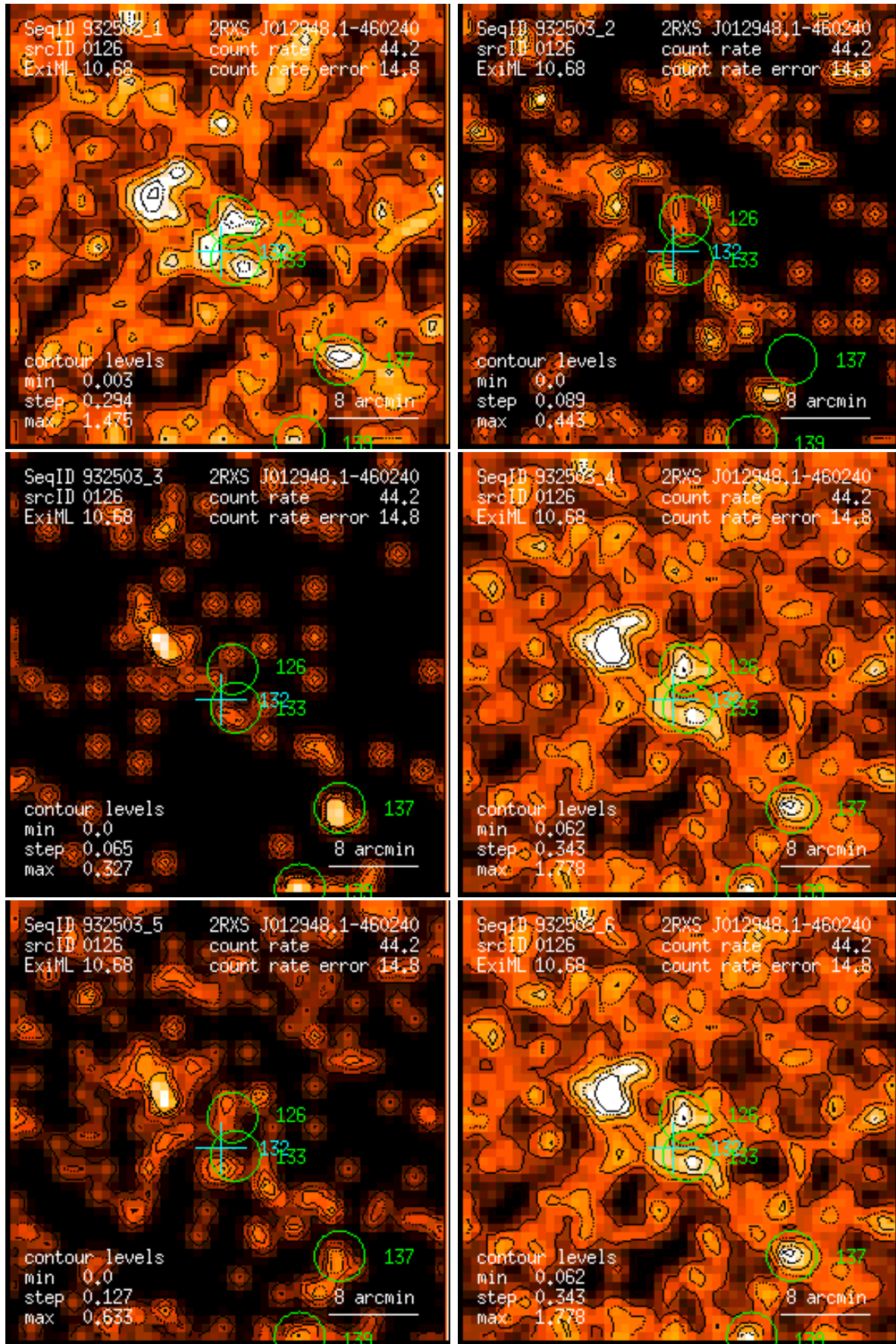
Figure 126: RASS 932503: detection 0126: band rate images, Gaussian filter: (1) PSPC channels 11 – 41, (2) 52 – 90, (3) 91 – 201, (4) 11 – 235, (5) 52 – 201, (6) 11 – 201. Broad band rates in counts/ks. Band rate contour levels in counts/ks/arcmin 2 .
