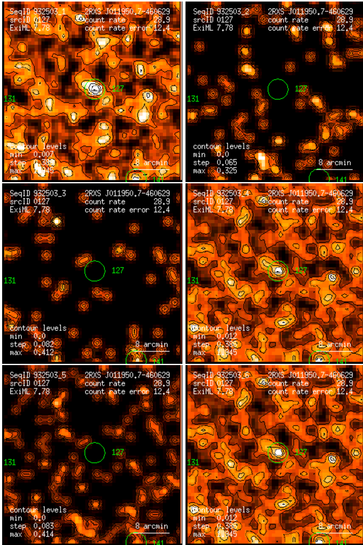
Figure 127: RASS 932503: detection 0127: band rate images, Gaussian filter: (1) PSPC channels 11 – 41, (2) 52 – 90, (3) 91 – 201, (4) 11 – 235, (5) 52 – 201, (6) 11 – 201. Broad band rates in counts/ks. Band rate contour levels in counts/ks/arcmin 2 .
