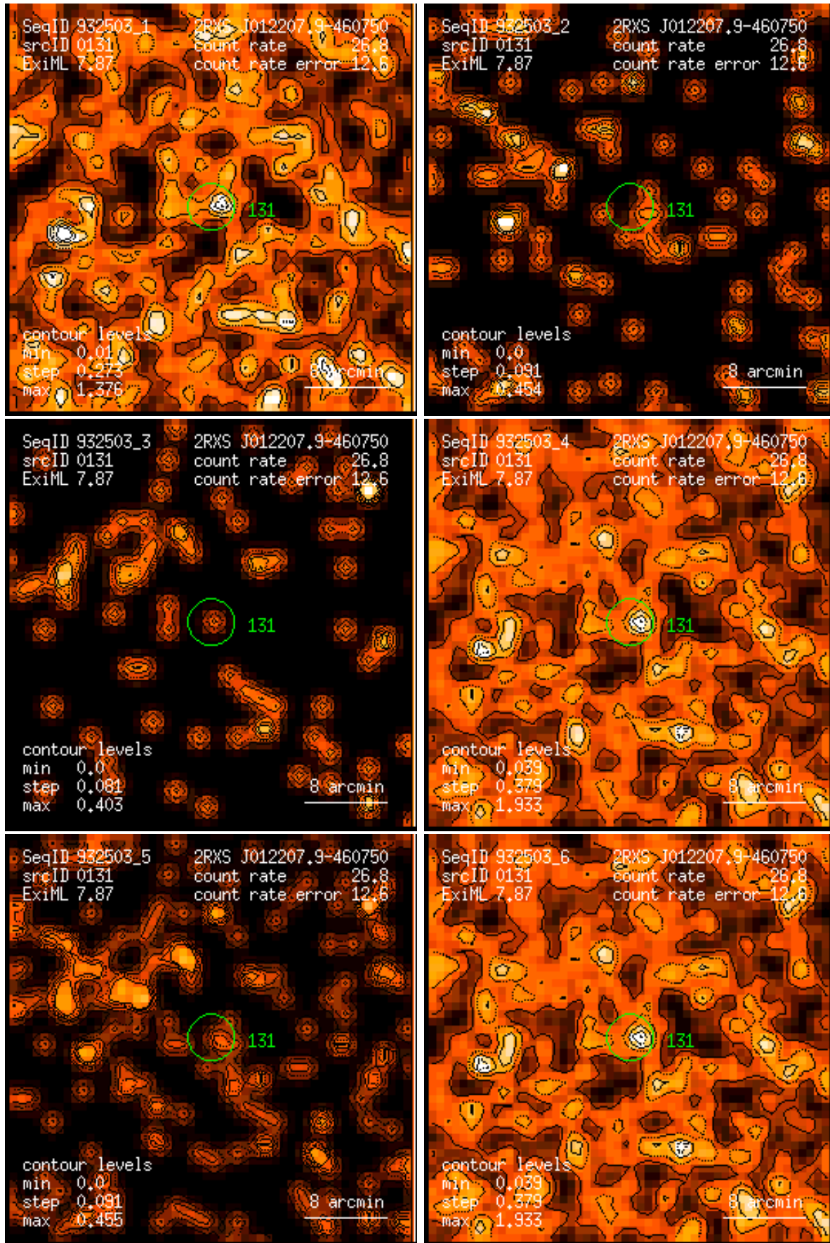
Figure 131: RASS 932503: detection 0131: band rate images, Gaussian filter: (1) PSPC channels 11 – 41, (2) 52 – 90, (3) 91 – 201, (4) 11 – 235, (5) 52 – 201, (6) 11 – 201. Broad band rates in counts/ks. Band rate contour levels in counts/ks/arcmin 2 .
