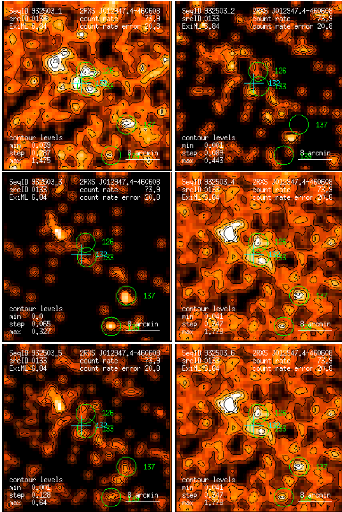
Figure 133: RASS 932503: detection 0133: band rate images, Gaussian filter: (1) PSPC channels 11 – 41, (2) 52 – 90, (3) 91 – 201, (4) 11 – 235, (5) 52 – 201, (6) 11 – 201. Broad band rates in counts/ks. Band rate contour levels in counts/ks/arcmin 2 .
