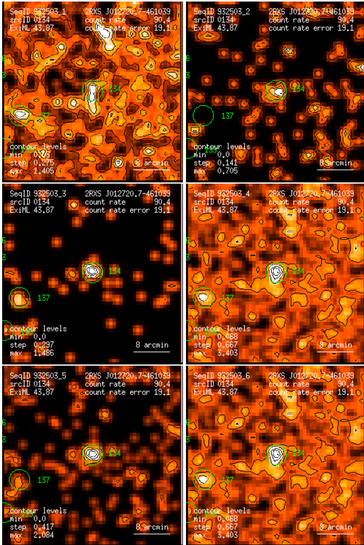
Figure 134: RASS 932503: detection 0134: band rate images, Gaussian filter: (1) PSPC channels 11 – 41, (2) 52 – 90, (3) 91 – 201, (4) 11 – 235, (5) 52 – 201, (6) 11 – 201. Broad band rates in counts/ks. Band rate contour levels in counts/ks/arcmin 2 .
