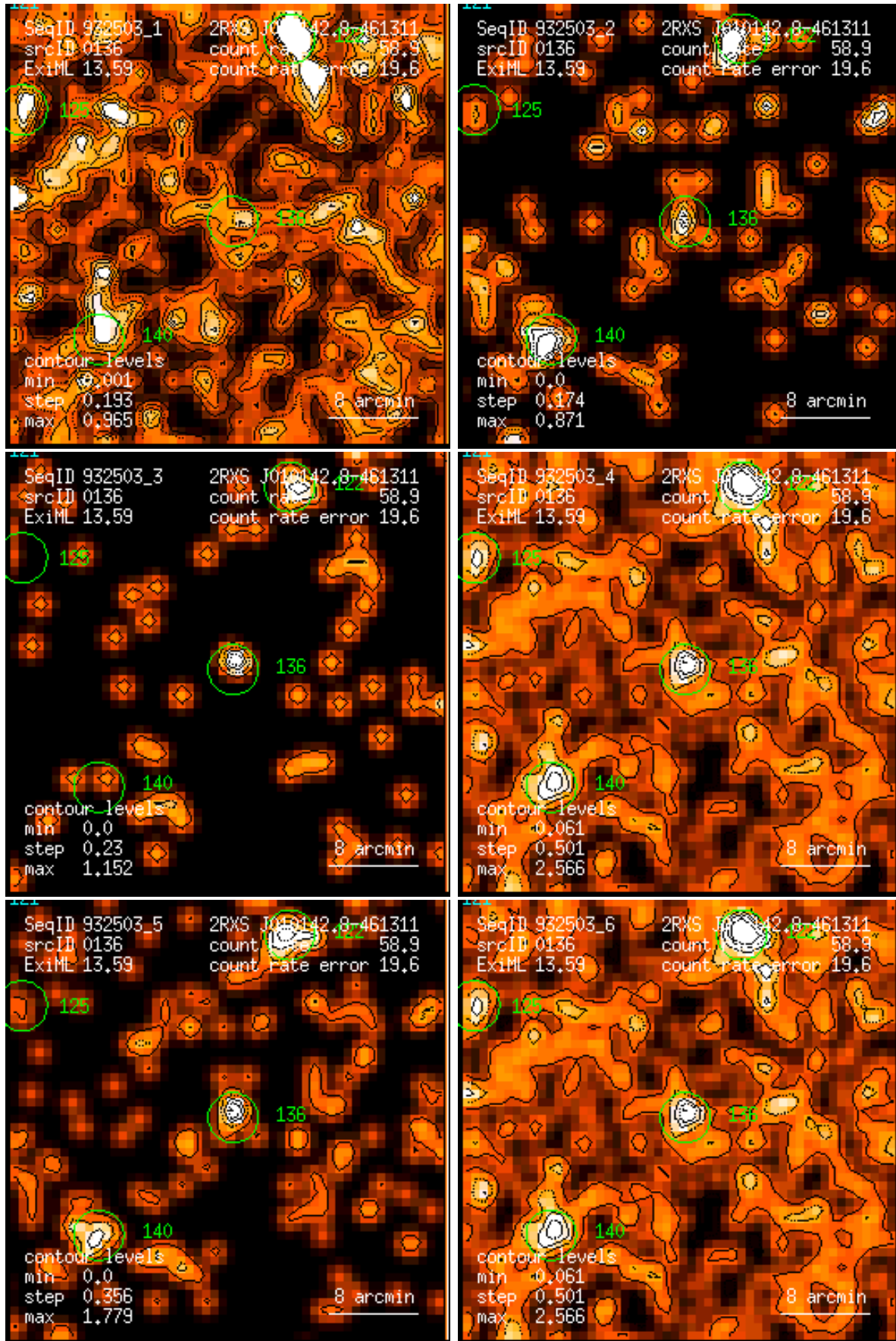
Figure 136: RASS 932503: detection 0136: band rate images, Gaussian filter: (1) PSPC channels 11 – 41, (2) 52 – 90, (3) 91 – 201, (4) 11 – 235, (5) 52 – 201, (6) 11 – 201. Broad band rates in counts/ks. Band rate contour levels in counts/ks/arcmin 2 .
