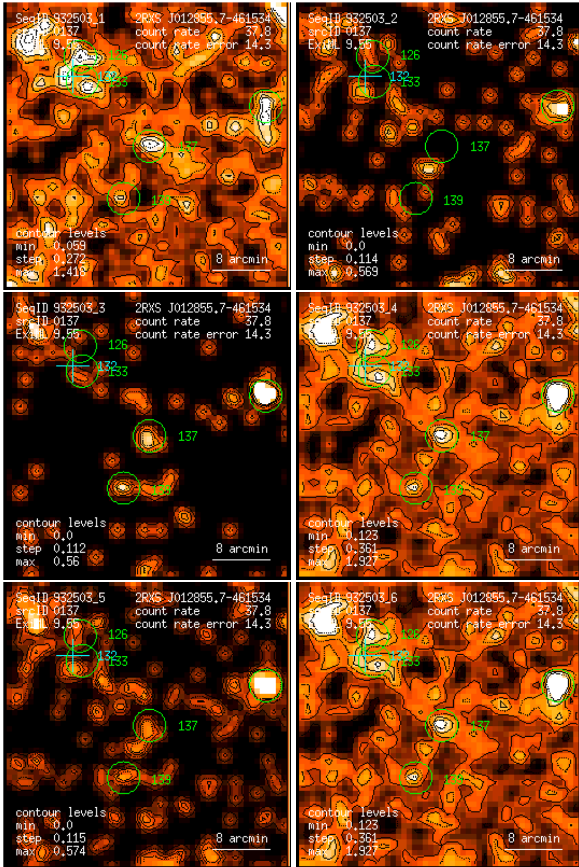
Figure 137: RASS 932503: detection 0137: band rate images, Gaussian filter: (1) PSPC channels 11 – 41, (2) 52 – 90, (3) 91 – 201, (4) 11 – 235, (5) 52 – 201, (6) 11 – 201. Broad band rates in counts/ks. Band rate contour levels in counts/ks/arcmin 2 .
