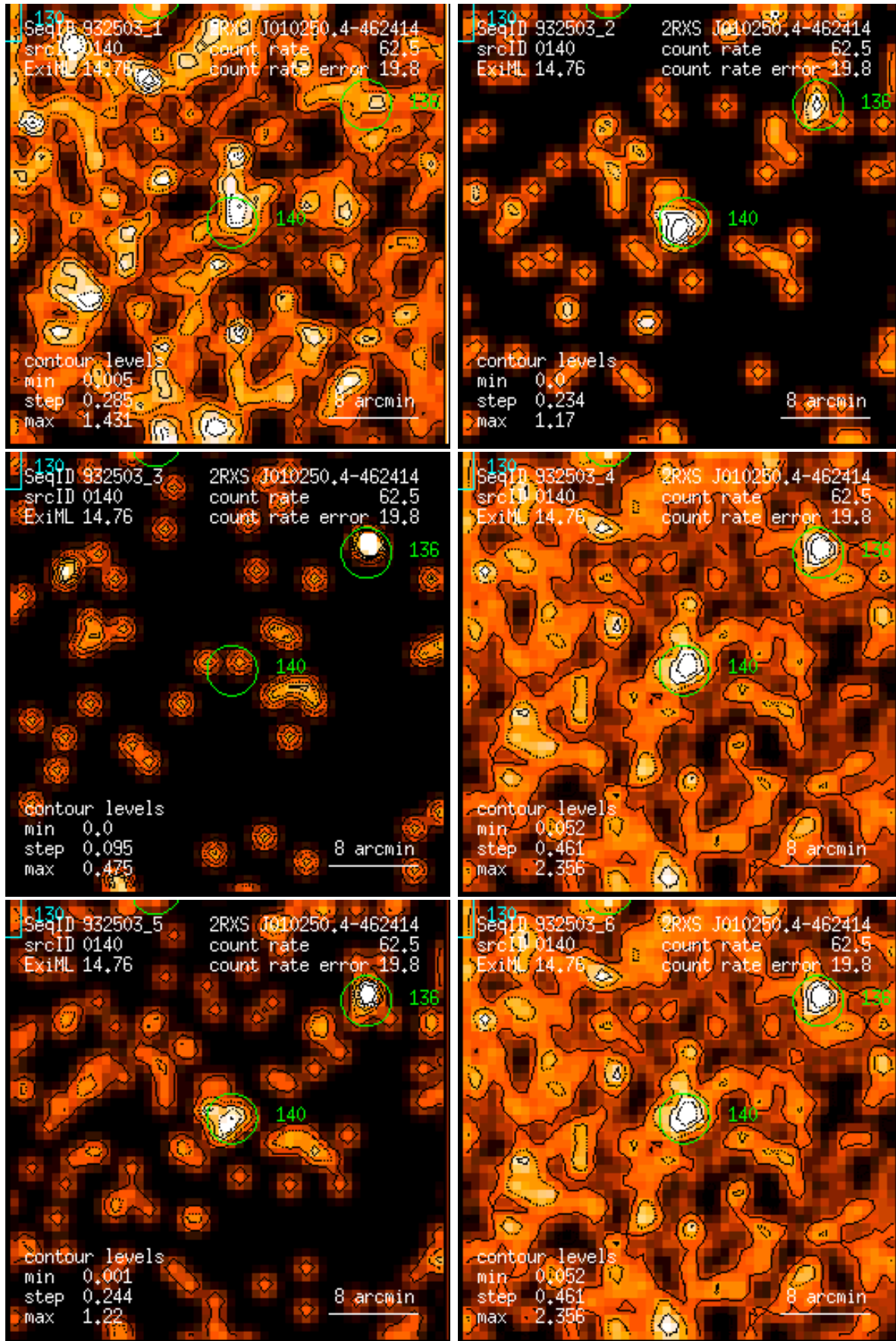
Figure 140: RASS 932503: detection 0140: band rate images, Gaussian filter: (1) PSPC channels 11 – 41, (2) 52 – 90, (3) 91 – 201, (4) 11 – 235, (5) 52 – 201, (6) 11 – 201. Broad band rates in counts/ks. Band rate contour levels in counts/ks/arcmin 2 .
