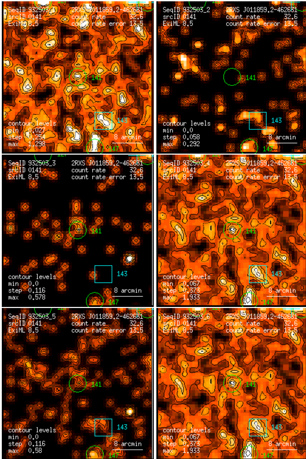
Figure 141: RASS 932503: detection 0141: band rate images, Gaussian filter: (1) PSPC channels 11 – 41, (2) 52 – 90, (3) 91 – 201, (4) 11 – 235, (5) 52 – 201, (6) 11 – 201. Broad band rates in counts/ks. Band rate contour levels in counts/ks/arcmin 2 .
