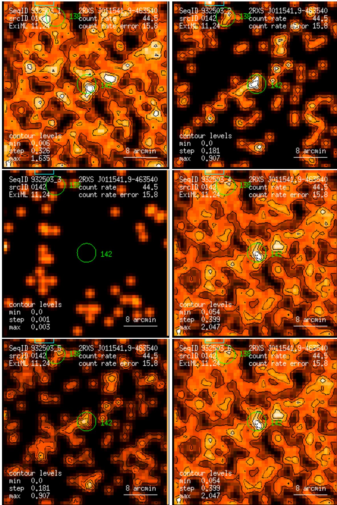
Figure 142: RASS 932503: detection 0142: band rate images, Gaussian filter: (1) PSPC channels 11 – 41, (2) 52 – 90, (3) 91 – 201, (4) 11 – 235, (5) 52 – 201, (6) 11 – 201. Broad band rates in counts/ks. Band rate contour levels in counts/ks/arcmin 2 .
